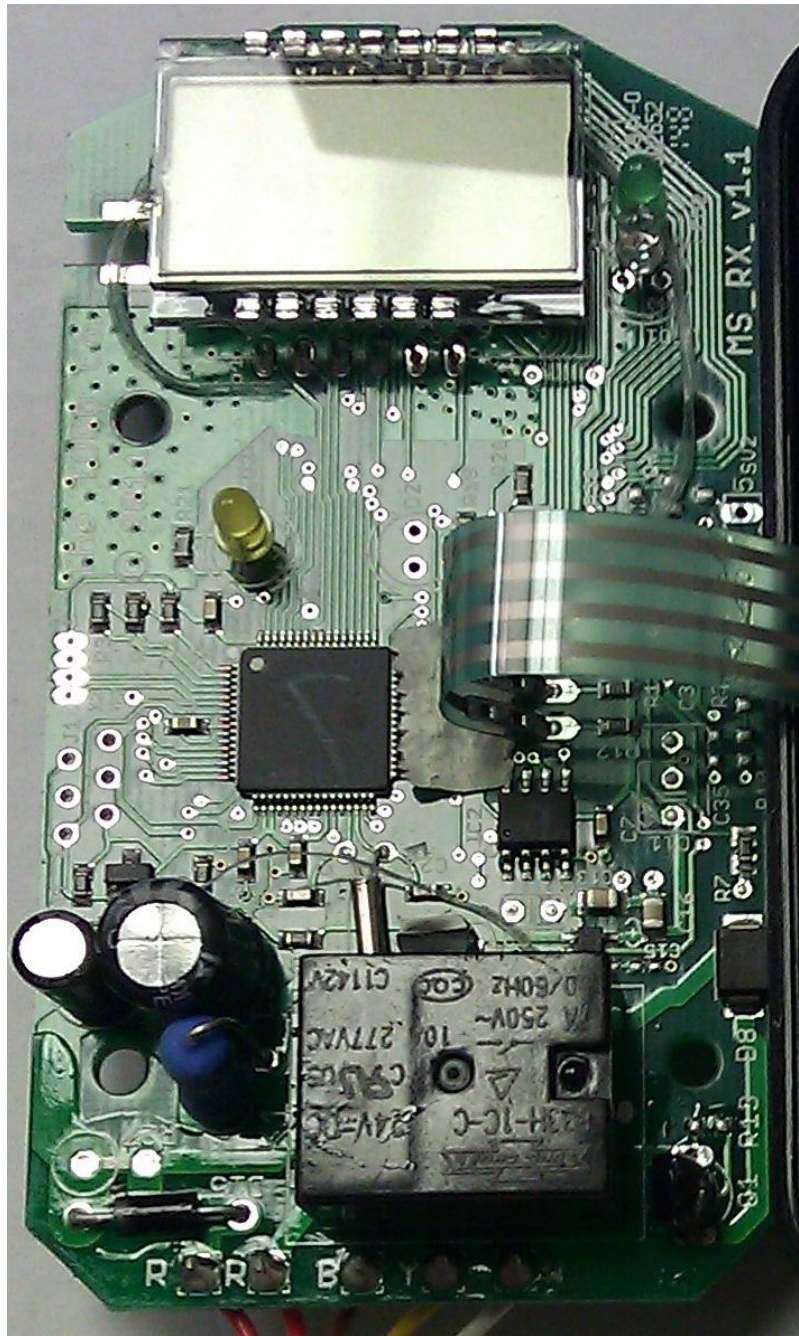
7.4 PCB Component View
