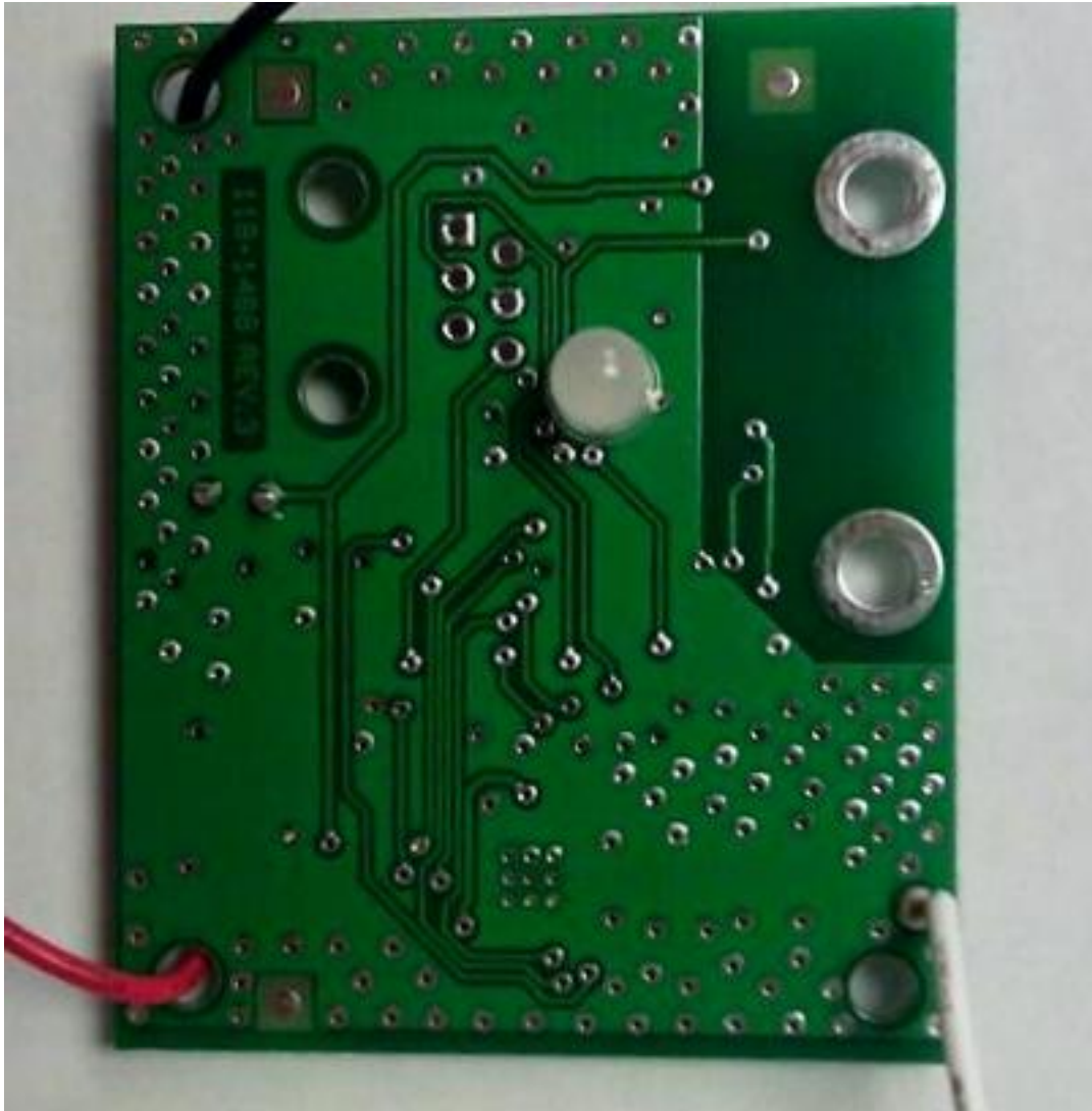
7.5 PCB Foil View
