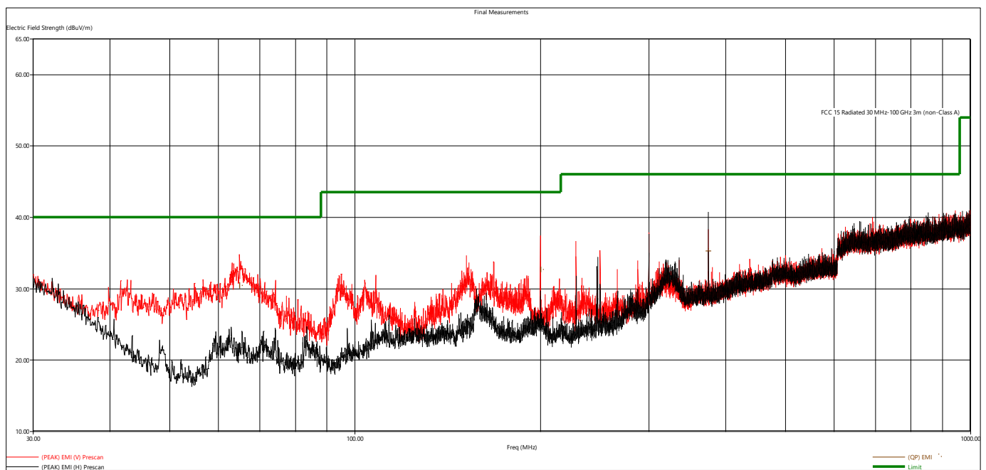
Figure 7 - Radiated Emissions Plot, 2EDR
