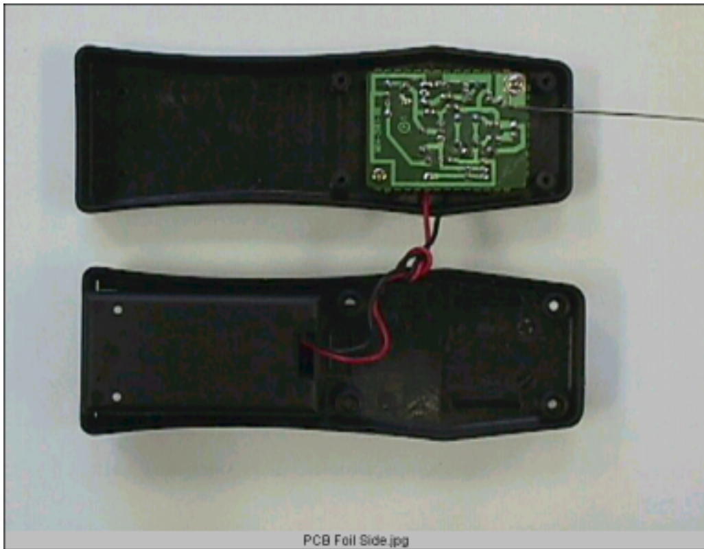
Expedite International - Transmitter PCB in case / foil side
