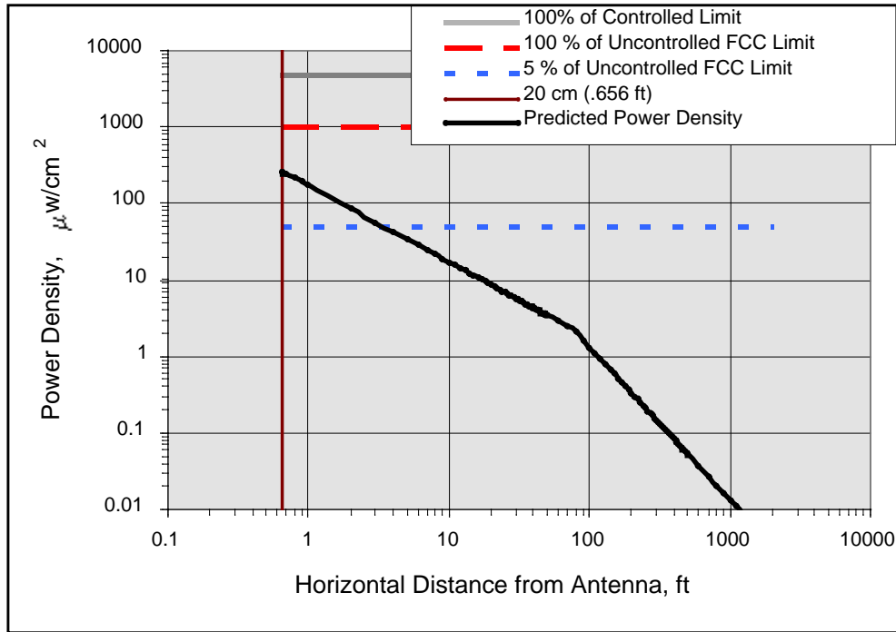
Figure 9.2 Uncontrolled MPE vs. Horizontal Distance
