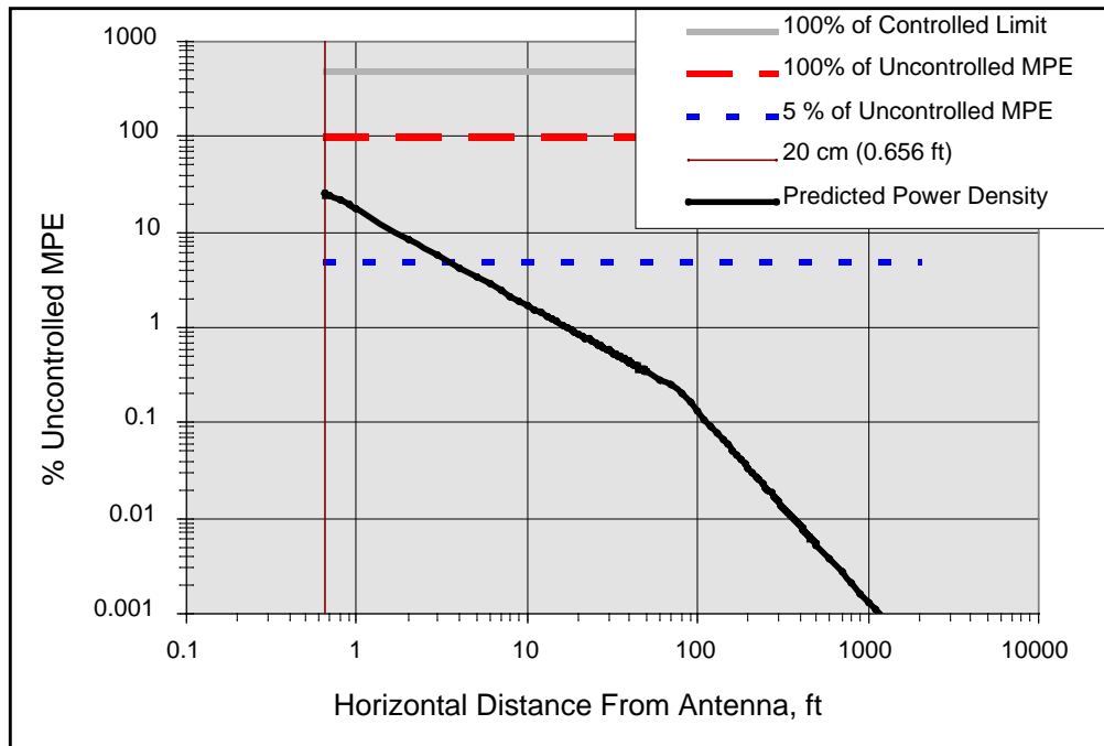
Figure 9.2 Uncontrolled MPE vs. Horizontal Distance
