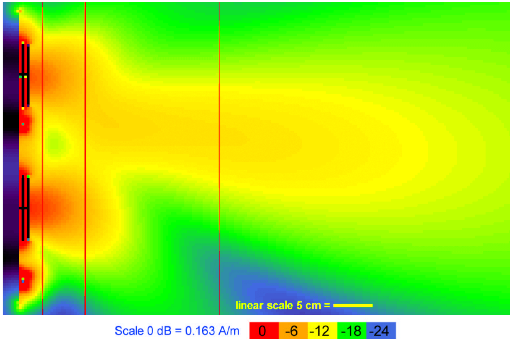
Figure 5.37. FDTD derived H-field of AT&T RU antenna in x-z plane compared to ANSI/IEEE exposure standard (Scan F, vertical plane through middle of left row of patches).
