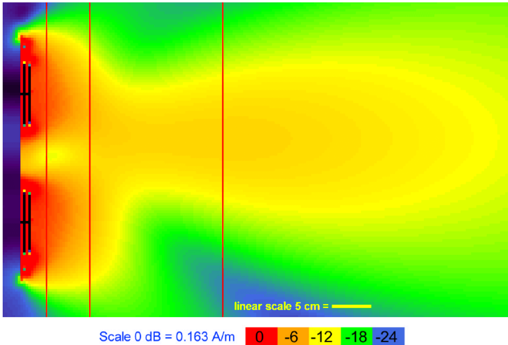
Figure 5.34. FDTD derived H-field of AT&T RU antenna in x-y plane compared to ANSI/IEEE exposure standard (Scan C, horizontal plane through middle of bottom patches).
