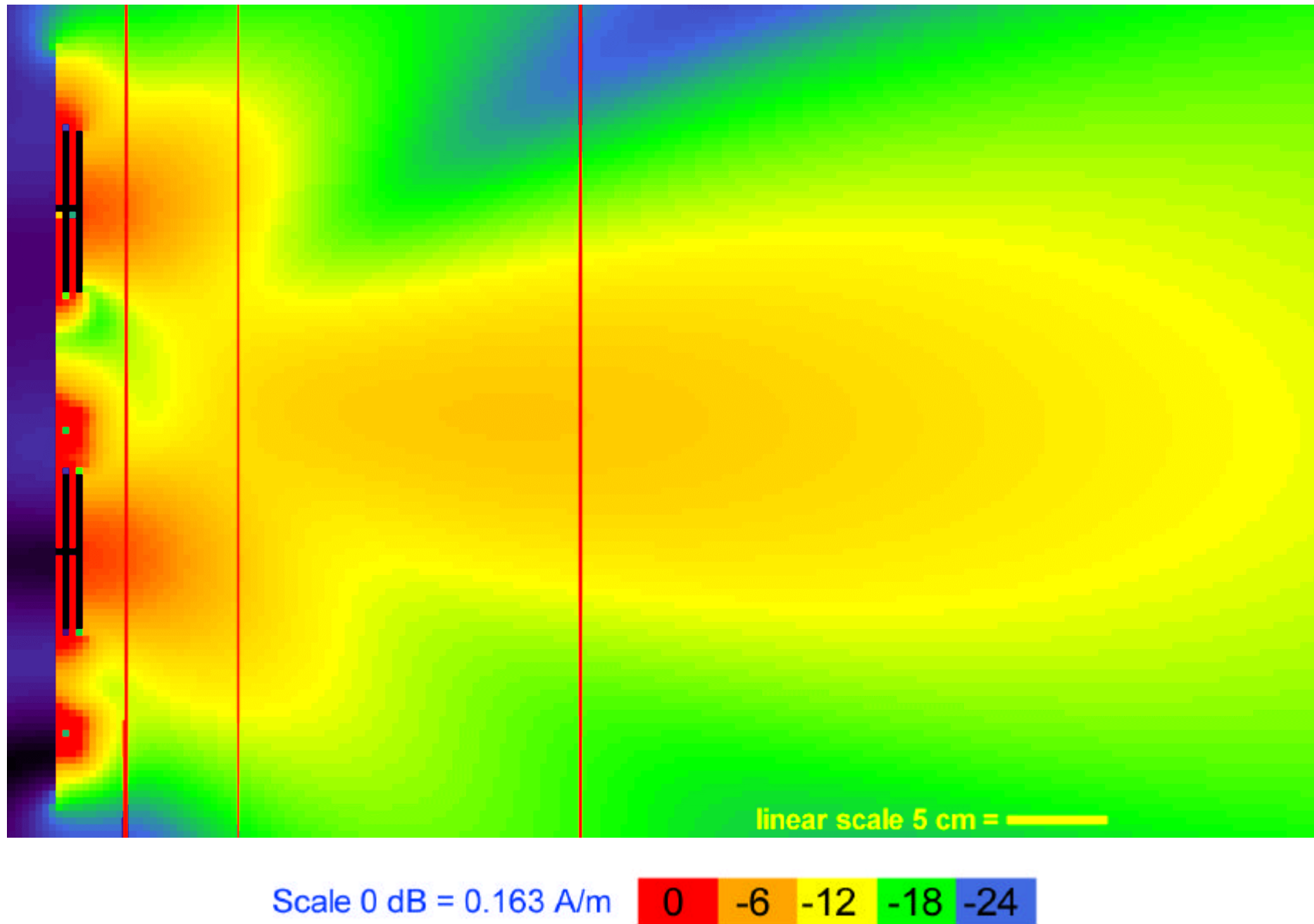
Figure 5.35. FDTD derived H-field of AT&T RU antenna in x-z plane compared to ANSI/IEEE exposure standard (Scan D, vertical plane through middle of right row of patches).
