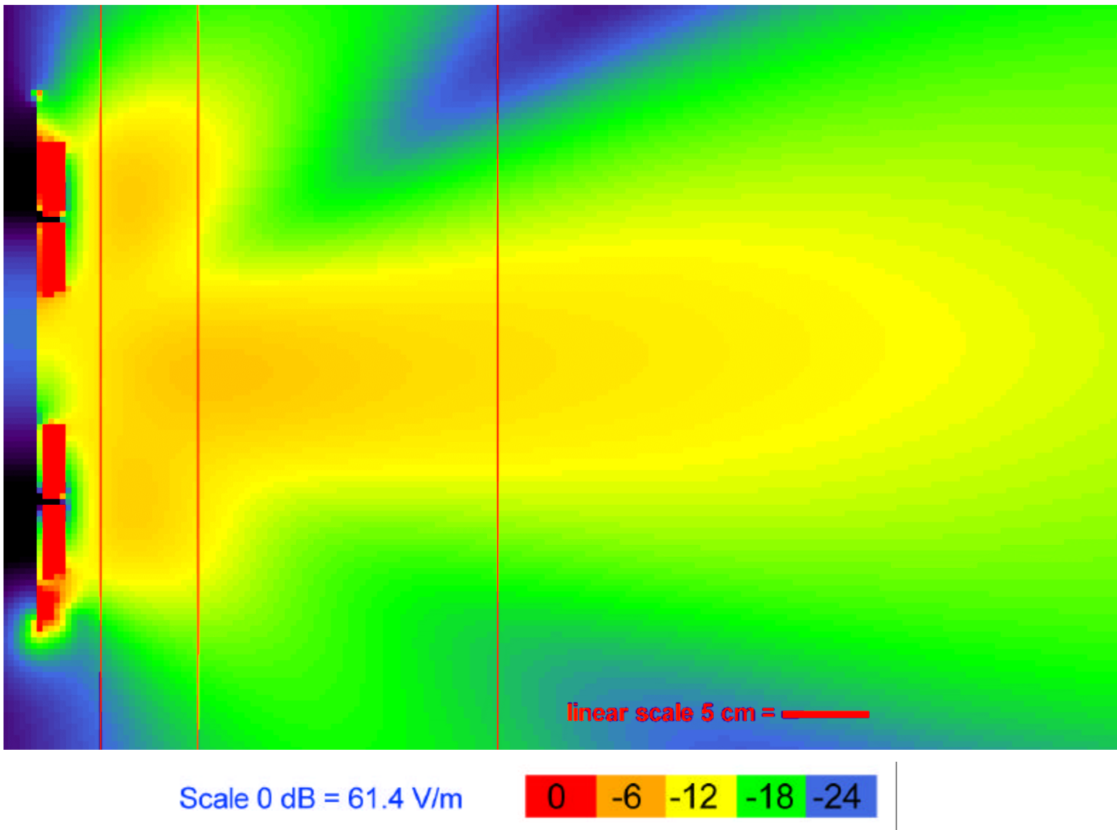
Figure 5.14. FDTD derived E-field of AT&T RU antenna in x-y plane compared to ANSI/IEEE exposure standard (Scan A, horizontal plane through middle of top patches).
