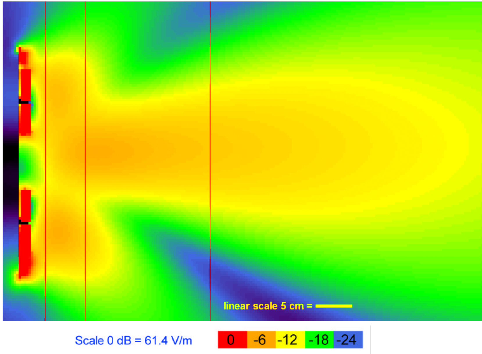
Figure 5.16. FDTD derived E-field of AT&T RU antenna in x-y plane compared to ANSI/IEEE exposure standard (Scan C, horizontal plane through middle of bottom patches).
