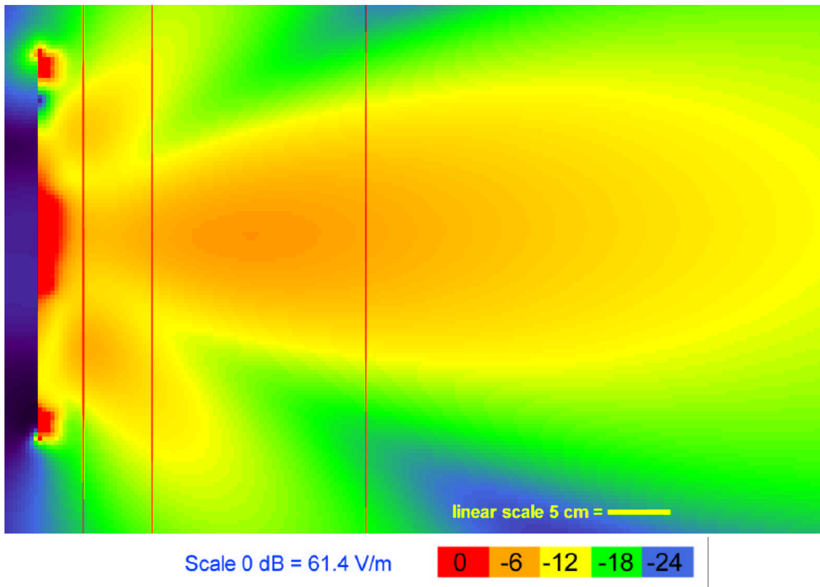
Figure 5.15. FDTD derived E-field of AT&T RU antenna in x-y plane compared to ANSI/IEEE exposure standard (Scan B, horizontal plane through middle of patch array).
