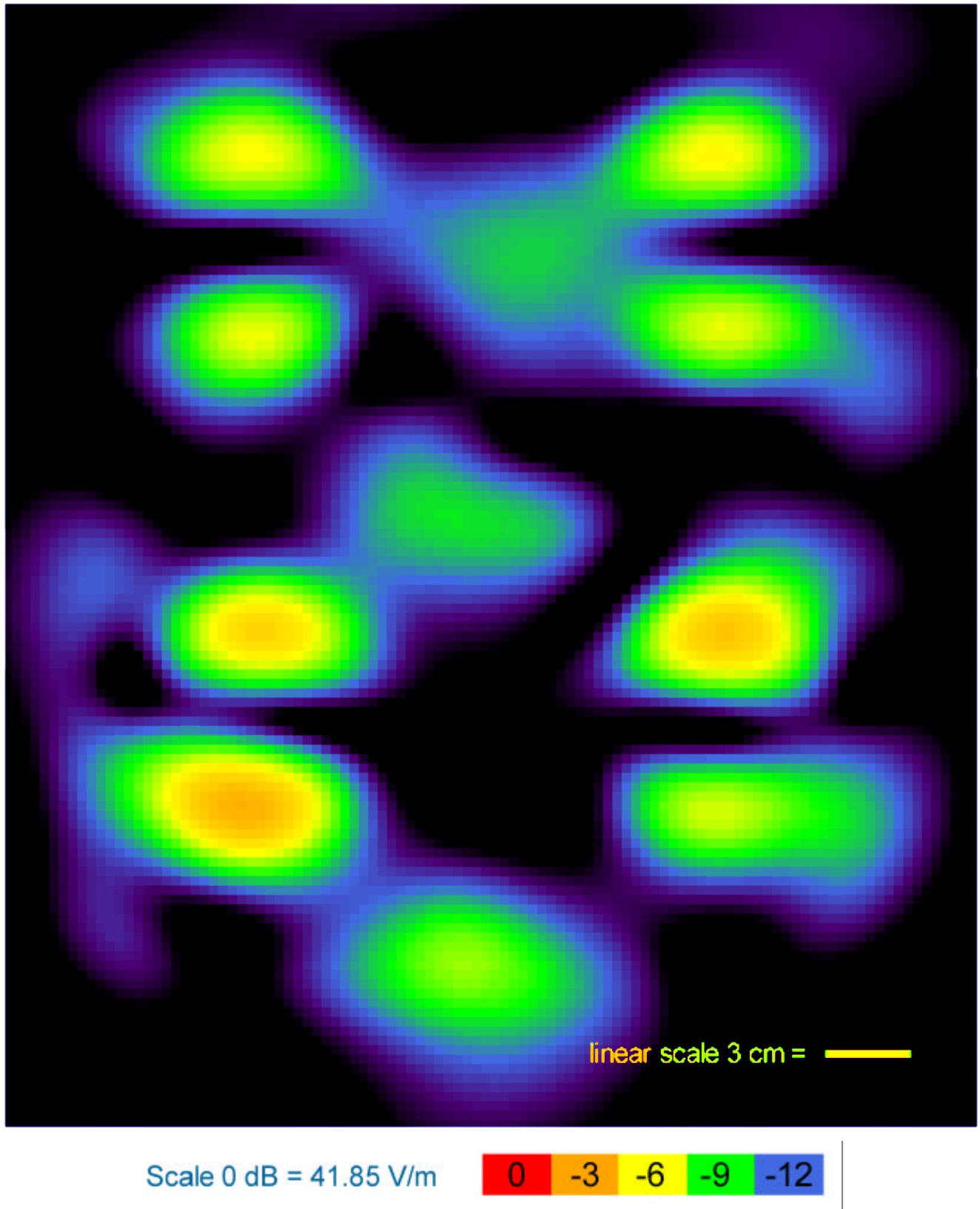
Figure 5.3. FDTD derived x component of E-field at of AT&T RU antenna in z-y plane (Scan H, 40 mm from ground plane of antenna for comparison with measured data).
