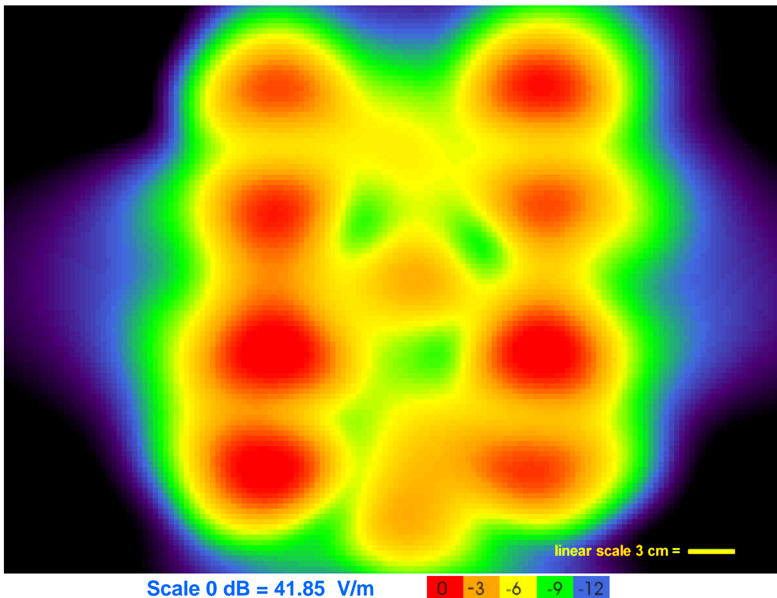
Figure 5.2. FDTD derived total E-field at of AT&T RU antenna in y-z plane (Scan H, 40 mm from ground plane of antenna for comparison with measured data).
