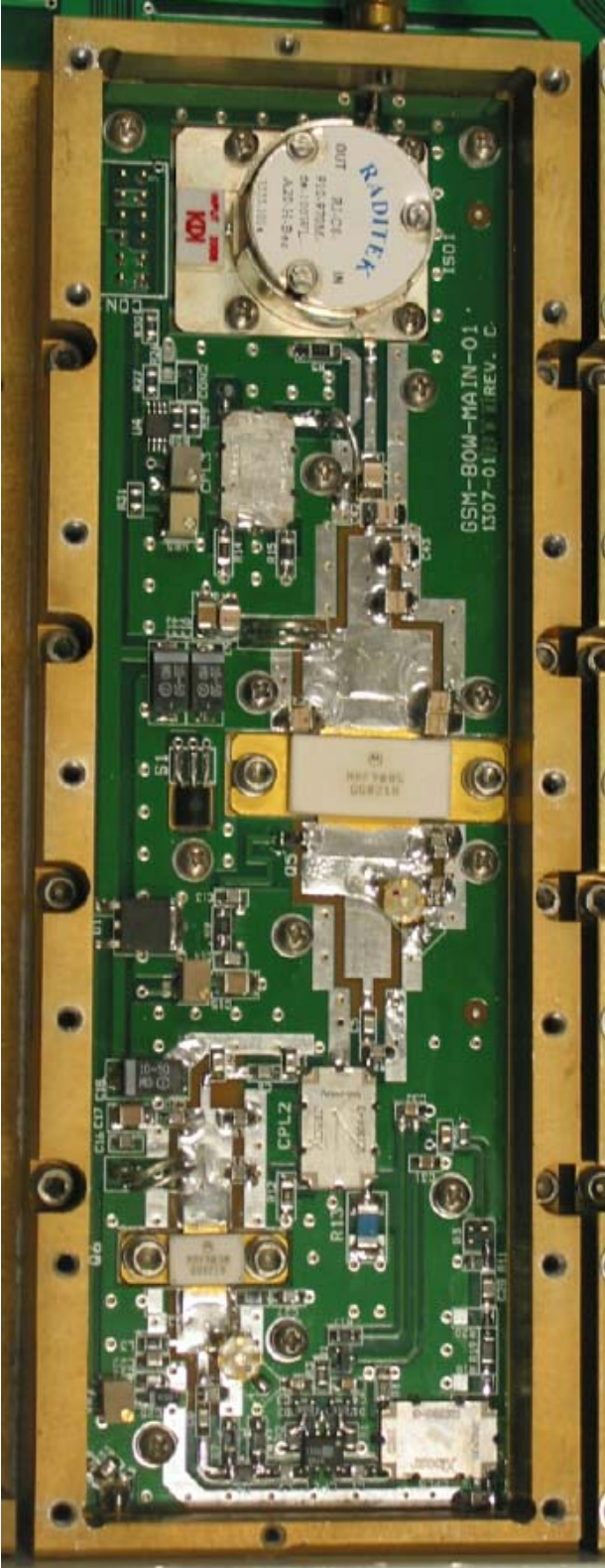
Amplifier
