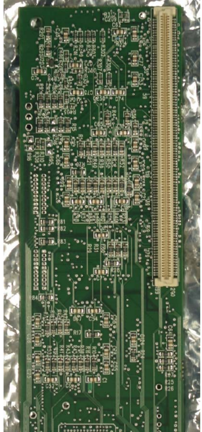
Radio Module, DSP Mezzanine Board Back Side
