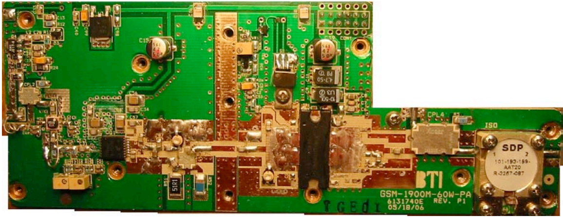
PA board
