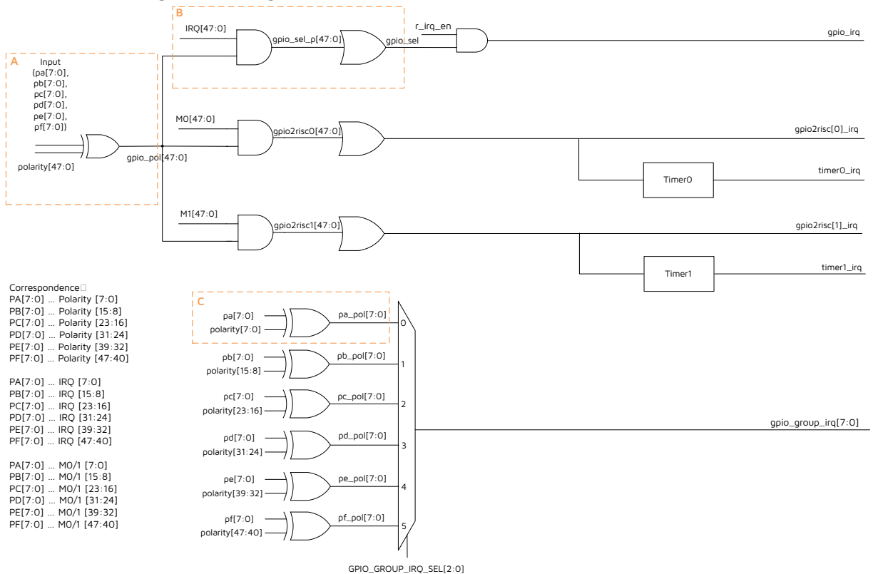
Figure 11-1 Logic Relationship between GPIO and Related Modules
