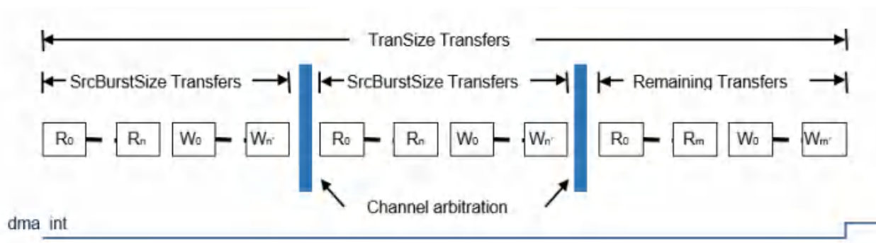
Figure 10-1 Example of DMA Data Transfers
