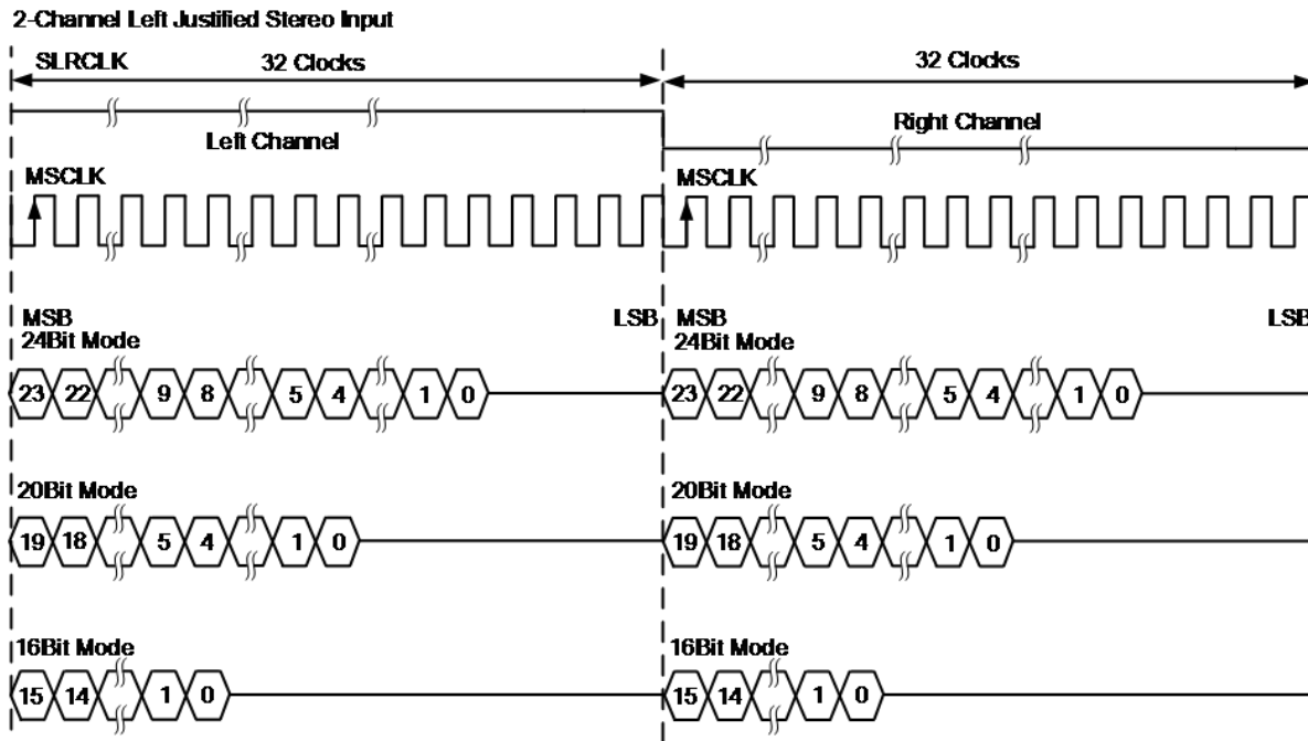
Figure 11-11 Timing Diagram of LJ Format
