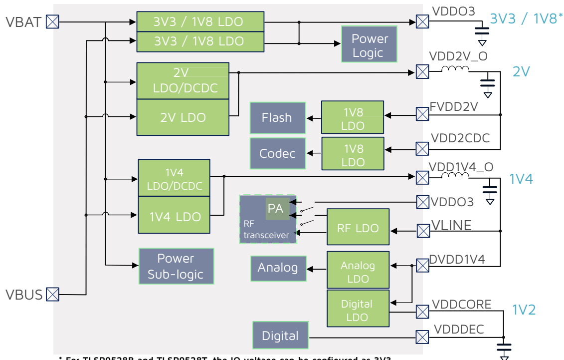
Figure 4-5 LDO and DCDC
