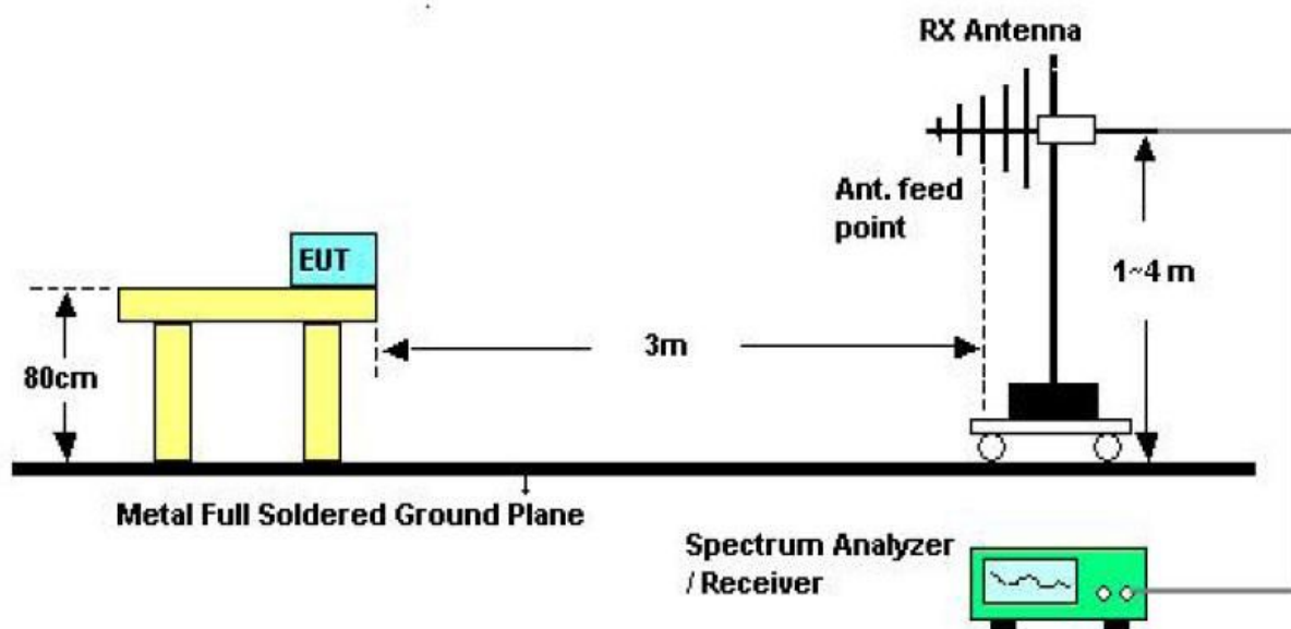
Above 30MHZ Test Setup
