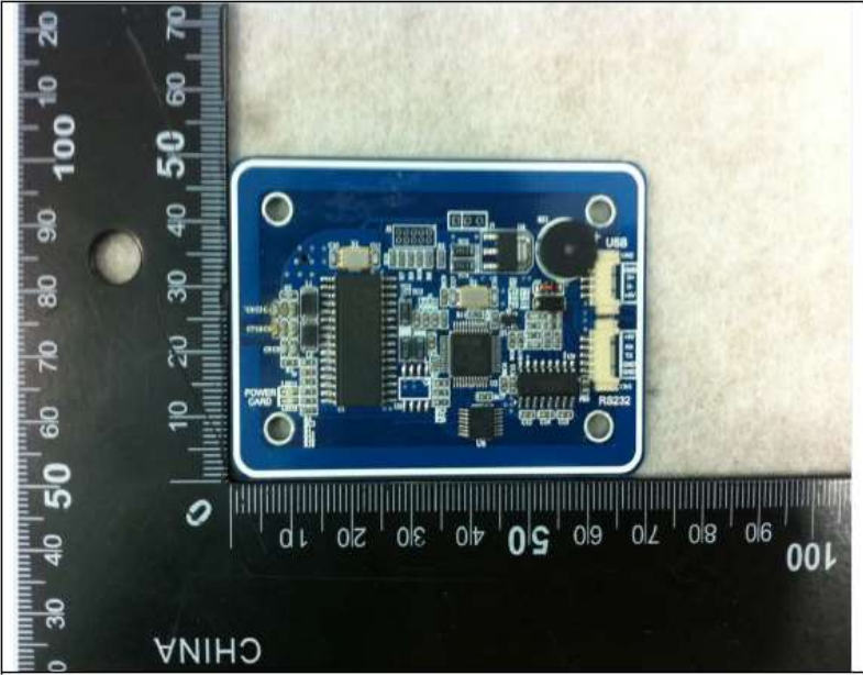
RFID reader PCB (Top)
