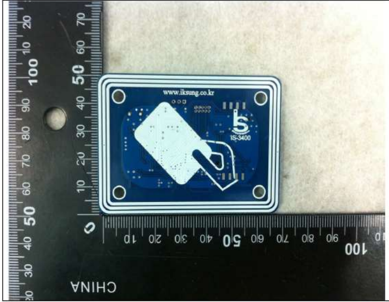
RFID reader PCB (Bottom)
