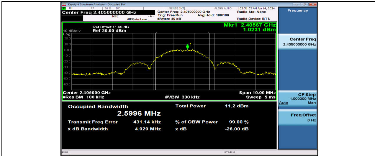
ZIGB-Ant1-2405
