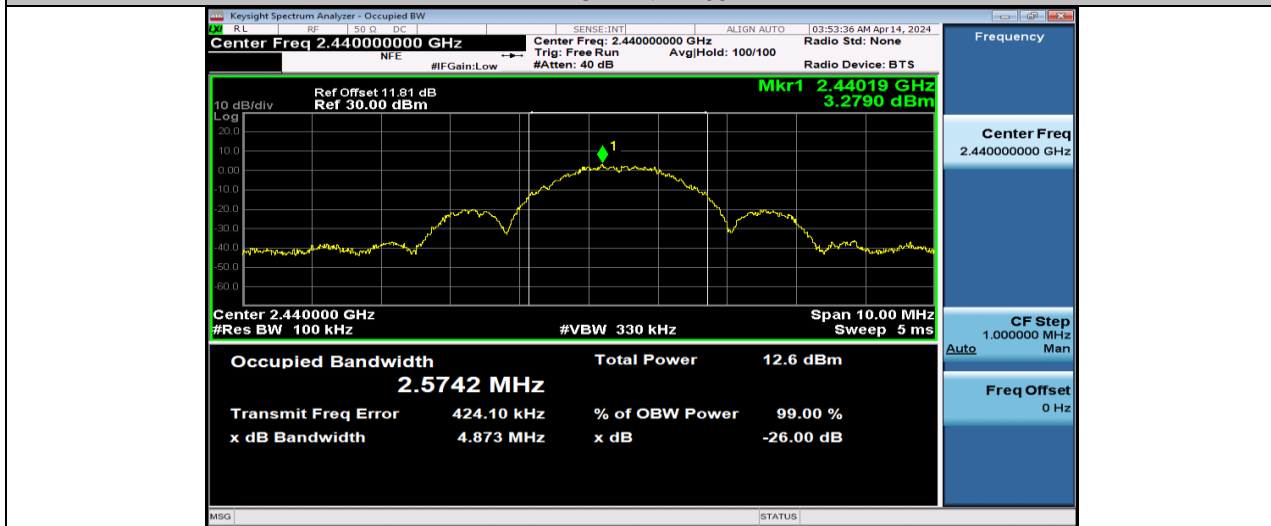
ZIGB-Ant1-2440
