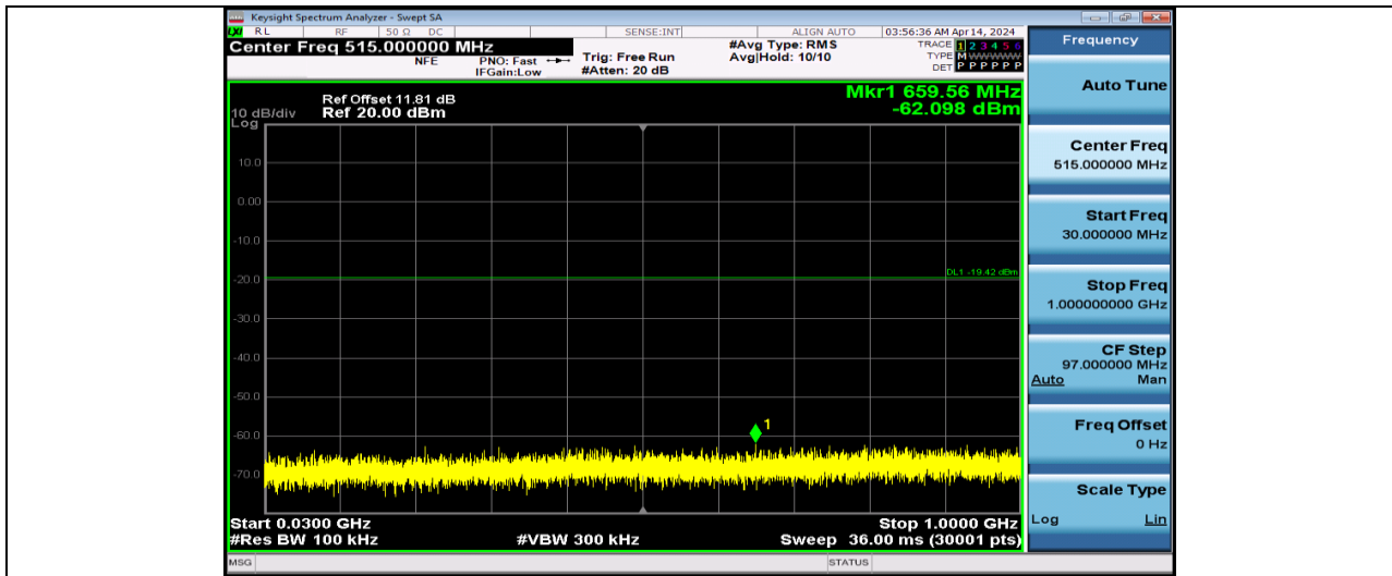
ZIGB-Ant1-2480-30~1000-PASS
