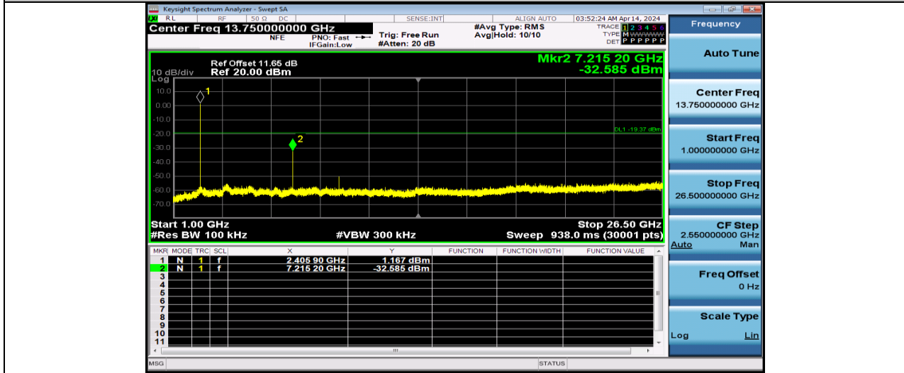
ZIGB-Ant1-2405-1000~26500-PASS
