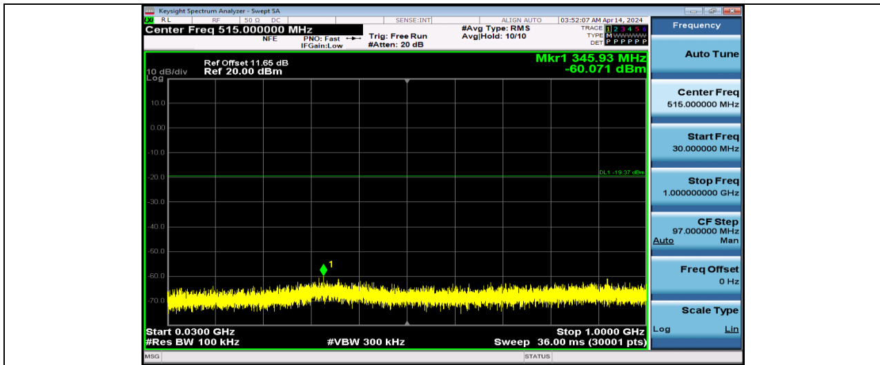
ZIGB-Ant1-2405-30~1000-PASS
