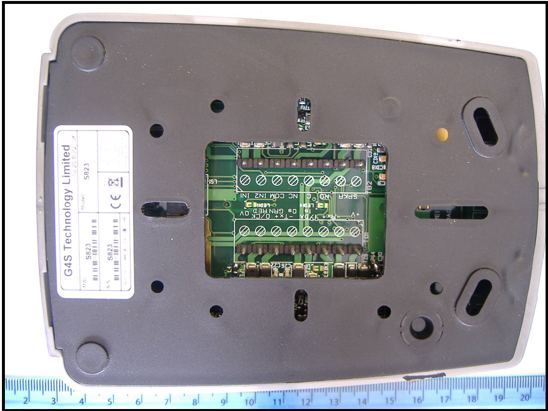
Rear Overview
