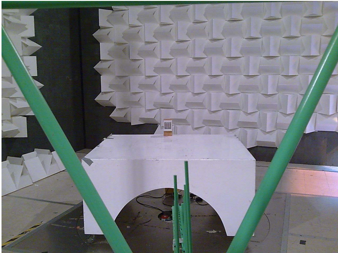
Test setup
