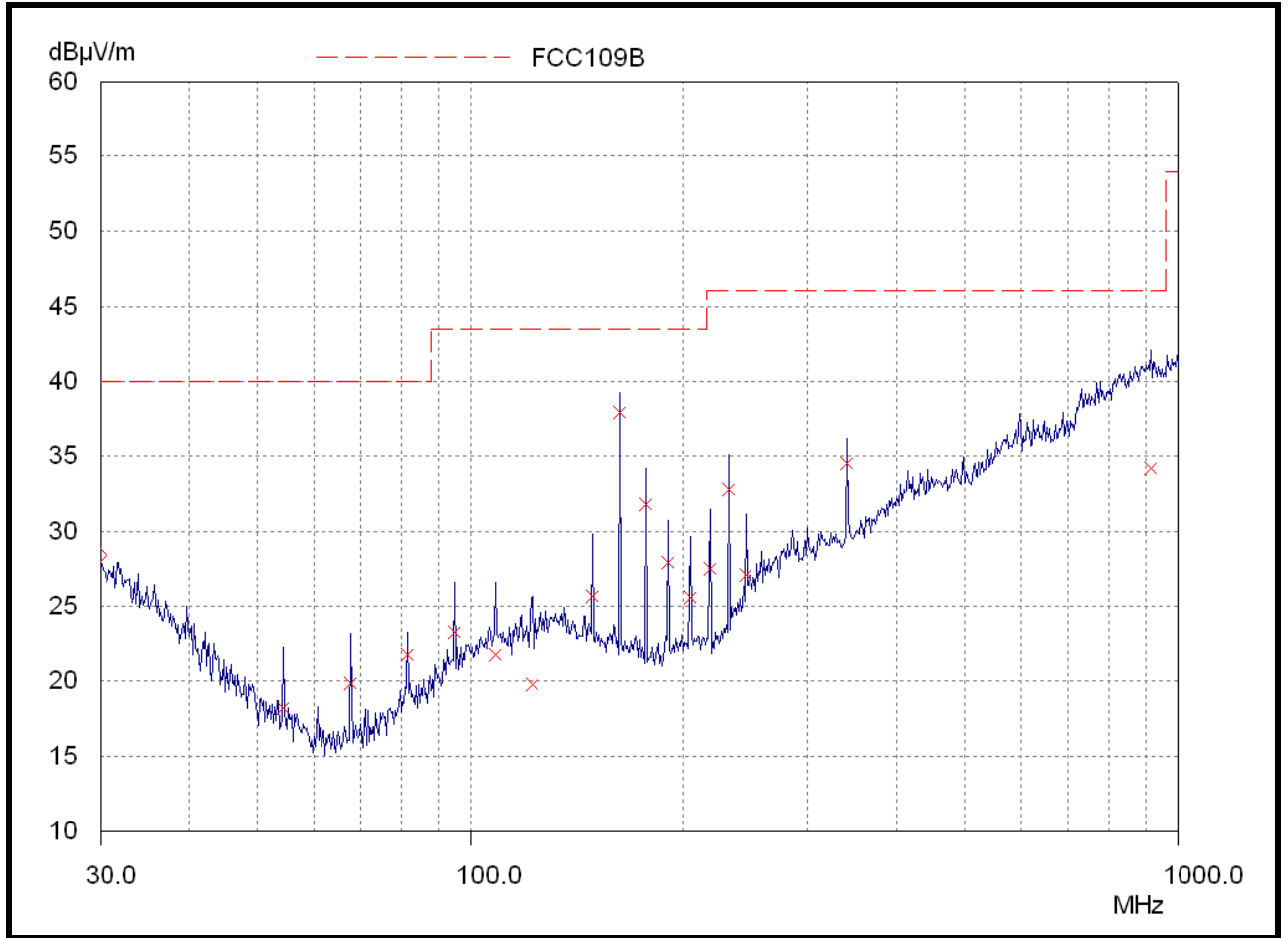
Radiated spurious emissions 30MHz to 1GHz
