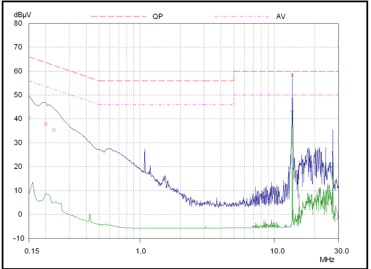
AC Powerline Conducted Emissions
