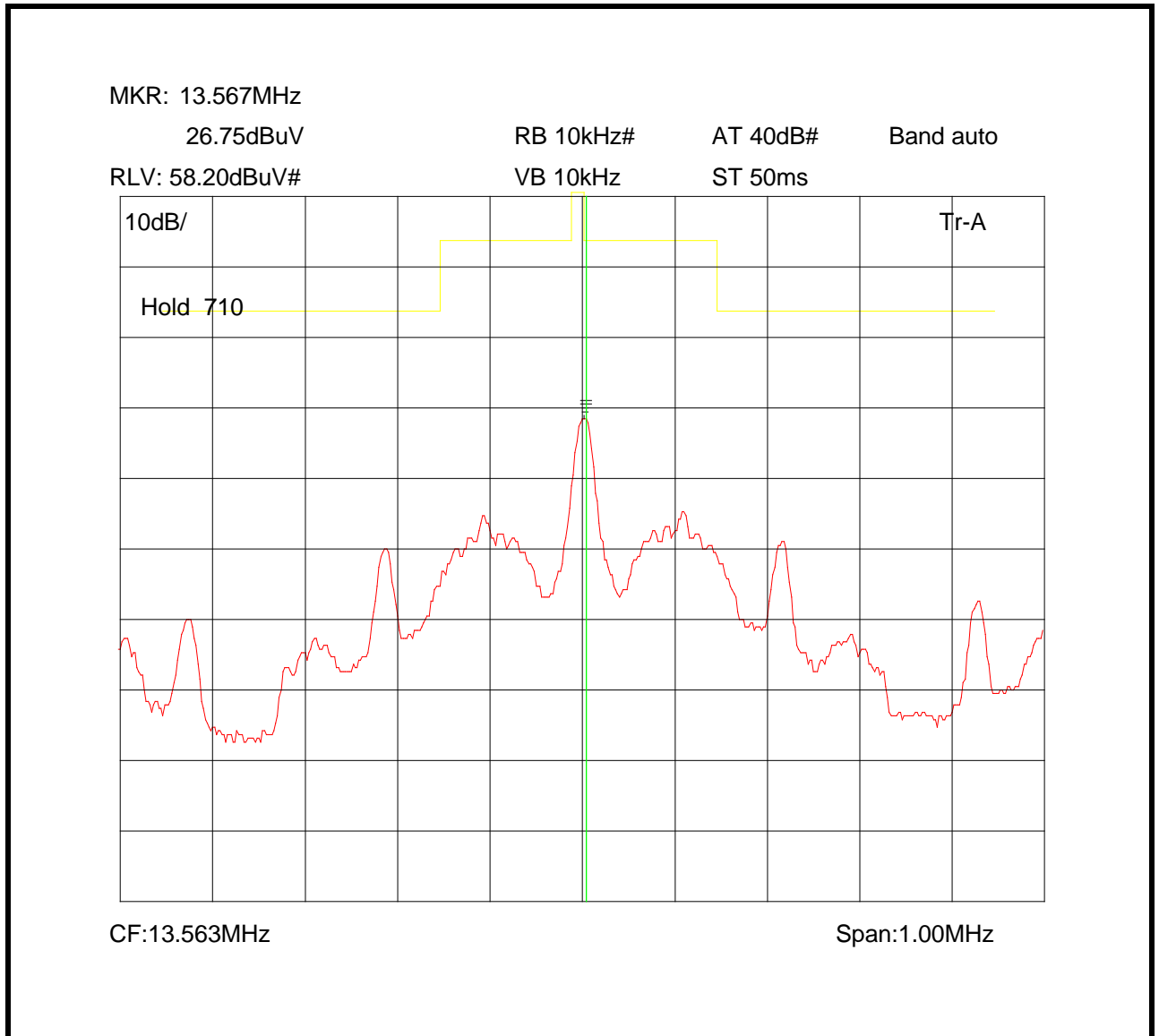
Emissions Mask at Tnom Vnom
