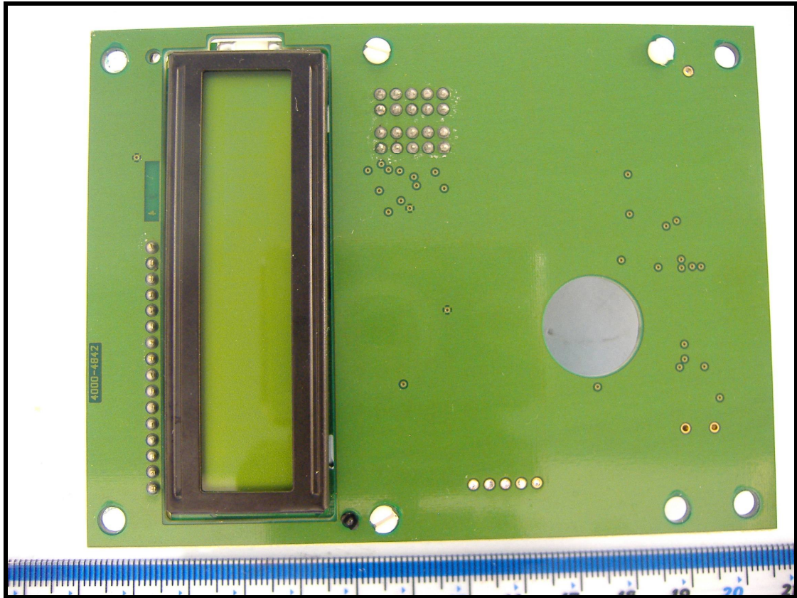
Display PCB Front Side
