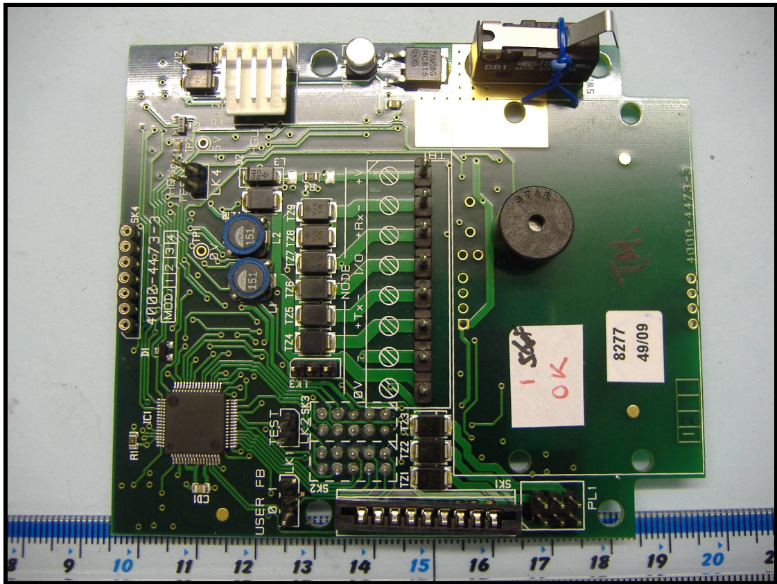
Control PCB Connector Side
