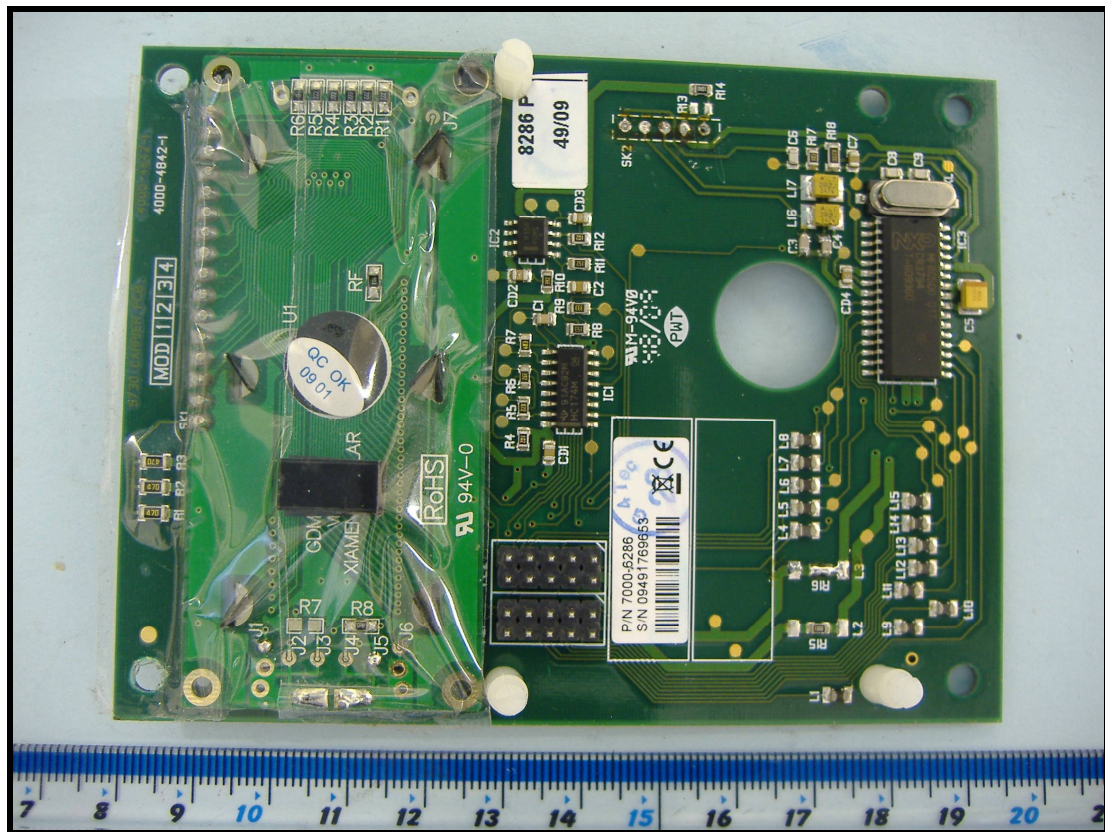
Display PCB Rear Side
