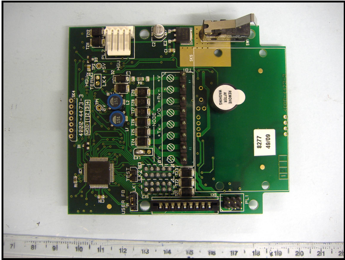
Main PCB Rear Side
