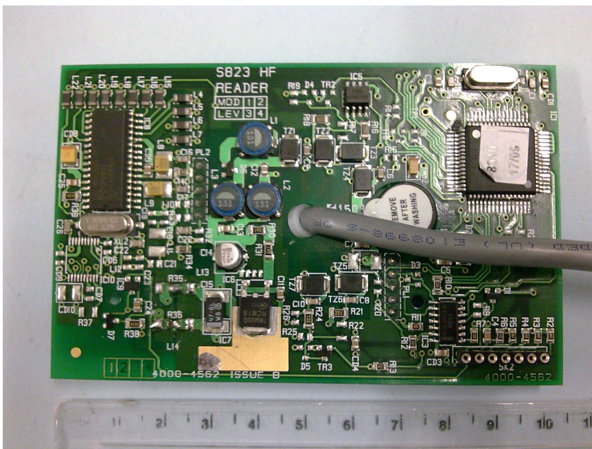
Top view PCB removed
