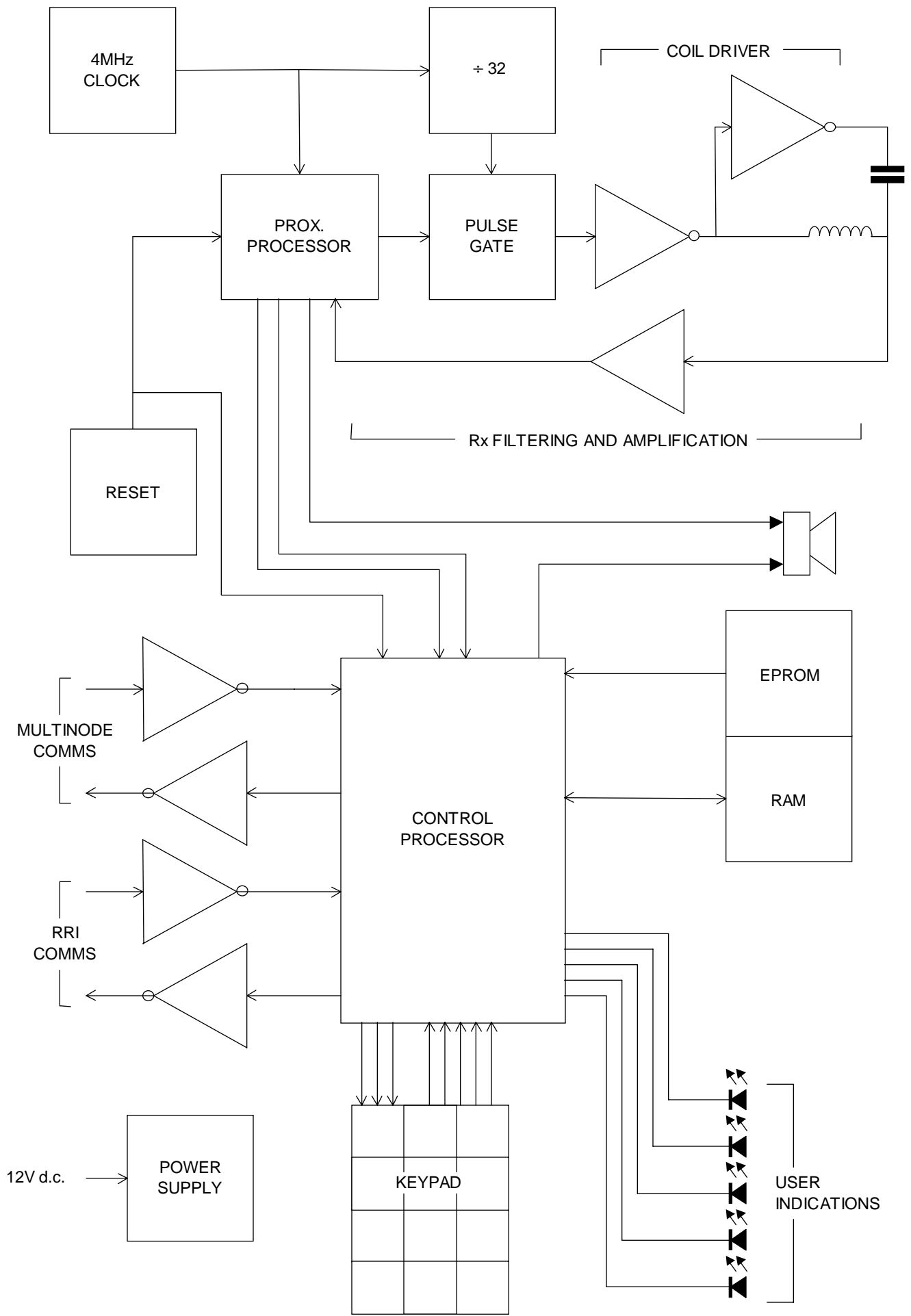
S675 Proximity Reader Block Diagram
