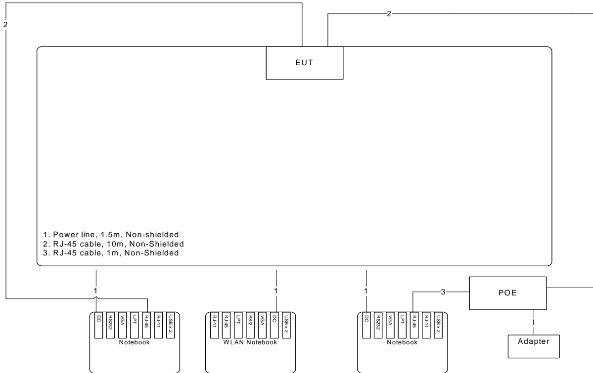
Test Configuration: Above 1GHz
