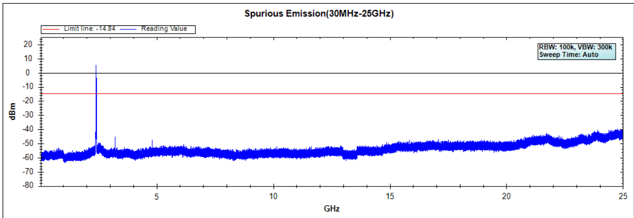
Channel 06 (2437MHz)
