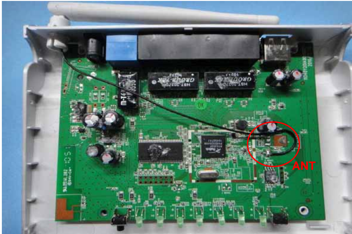
Internal Photo (Antenna gain 2.35 dBi)
