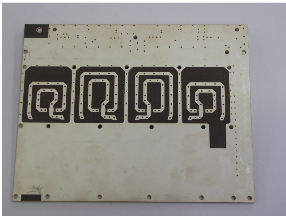
FILTER BOTTOM
