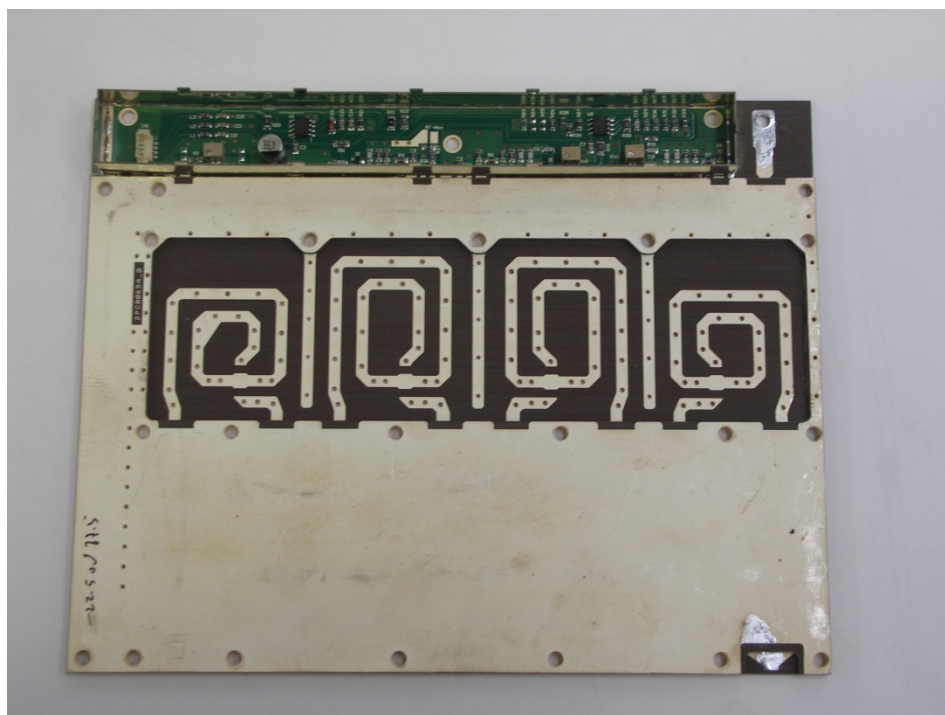
FILTER BOTTOM
