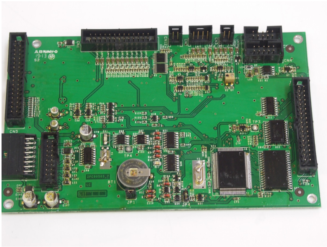
CPU BOTTOM
