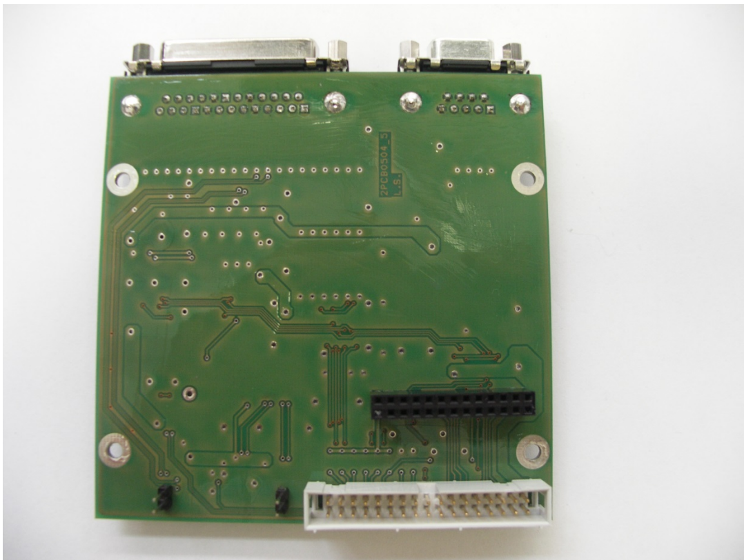
TCTS BOTTOM
