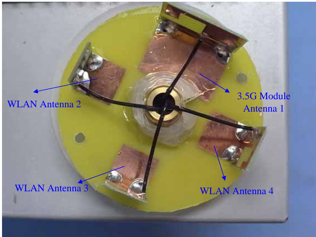
Figure 3 Antenna View
