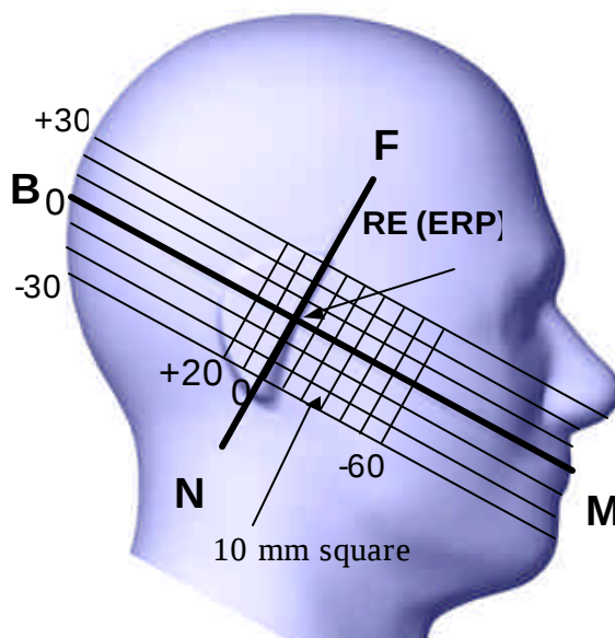
Figure 6. EUT Head Position
