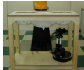
Figure 11. SAM Phantom
