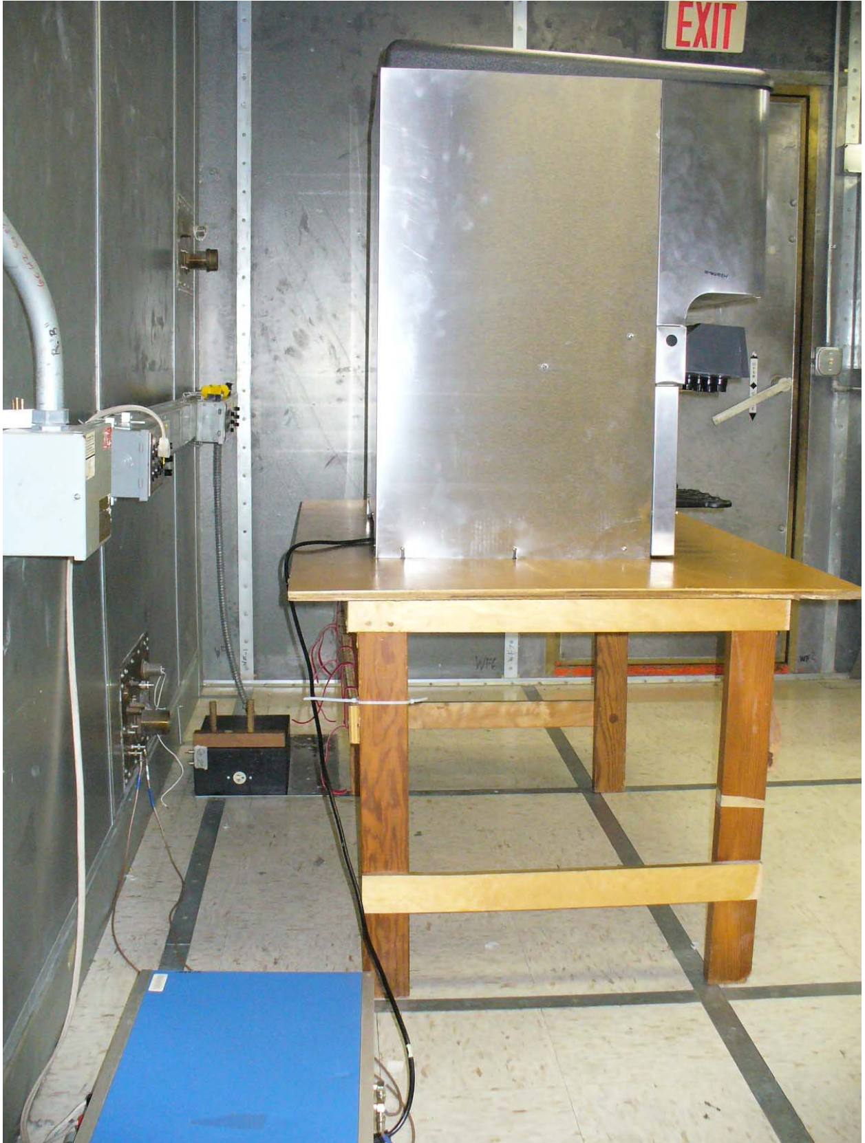
Figure 5: Power Line Conducted Emissions – Side View
