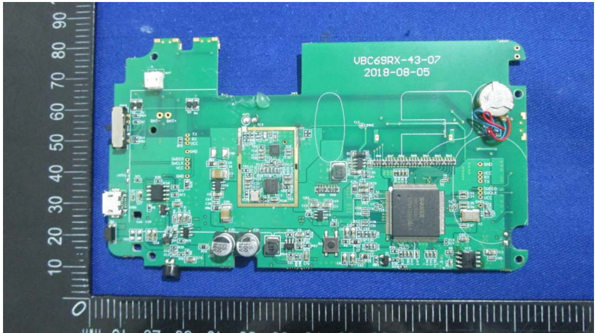
EUT –Main Board Unshielded Top View
