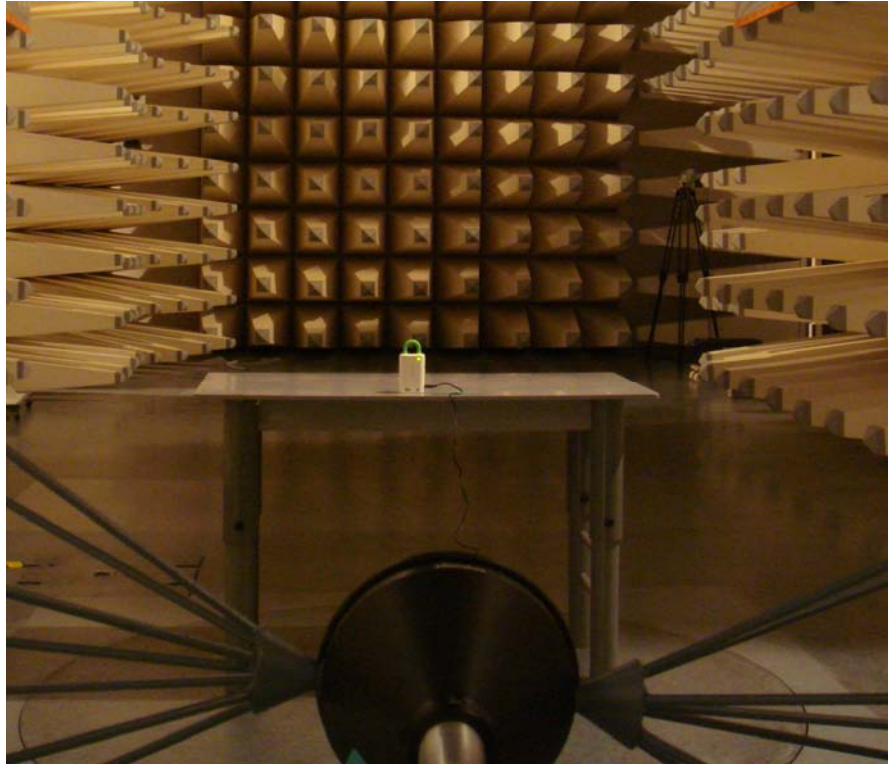
Radiated emission Test setup Photo
