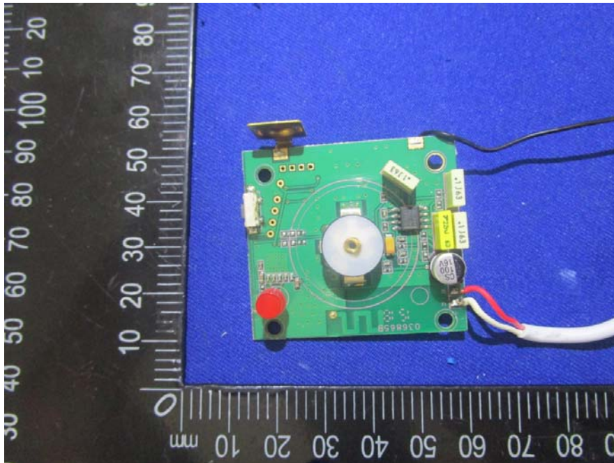
EUT – Transmit Unit Pcb Top View
