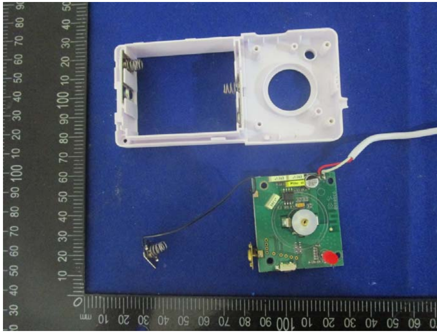
EUT – Transmit Unit Uncover View
