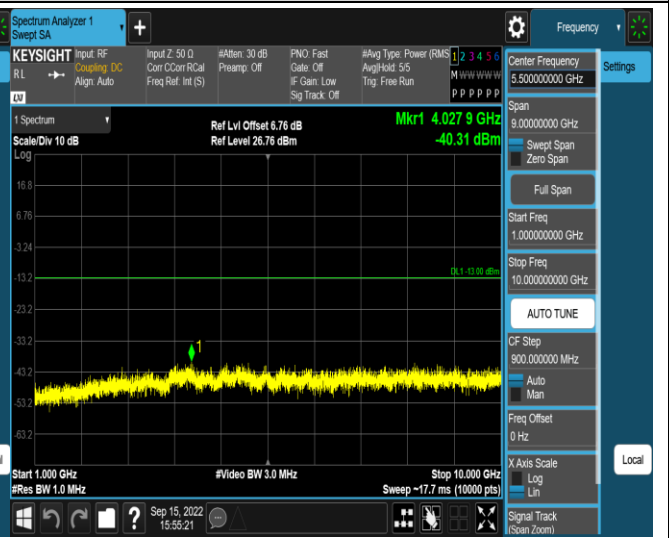
Band17-10MHz-16QAM-23800-1RB#0-Range2:1000~ 10000MHz
