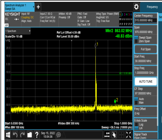
Band17-10MHz-16QAM-23800-1RB#0-Range1:30 ~1000MHz
