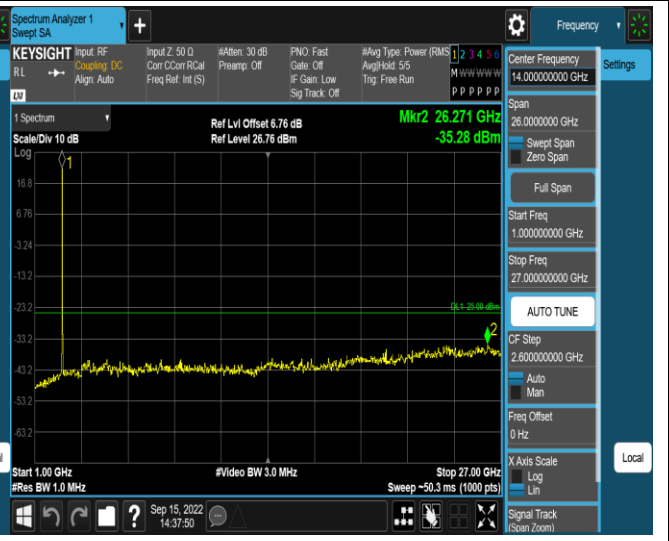
Band7-20MHz-16QAM-21100-1RB#0-Range2:1000~27000MHz
