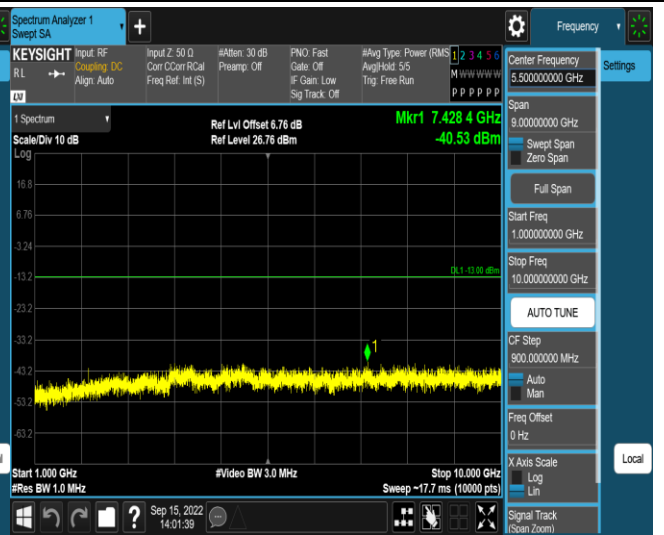
Band5-10MHz-QPSK-20525-1RB#0-Range2:1000~10000MHz
