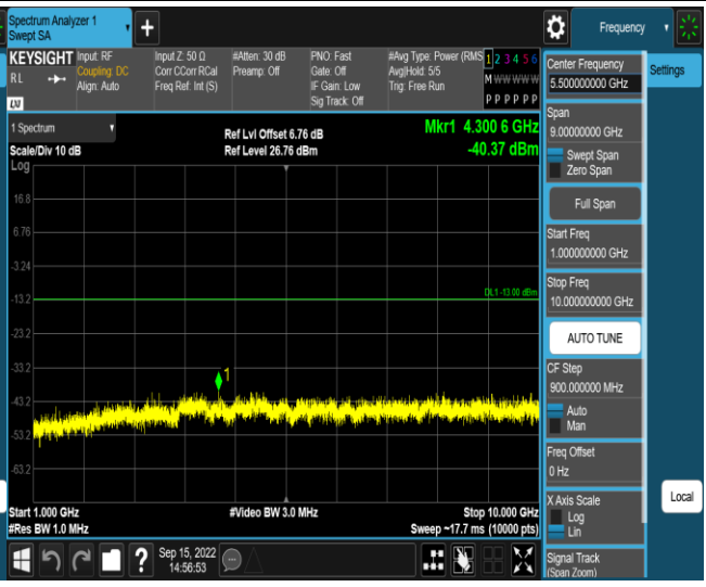
Band12-1.4MHz-16QAM-23017-1RB#0-Range2:1000~10000MHz
