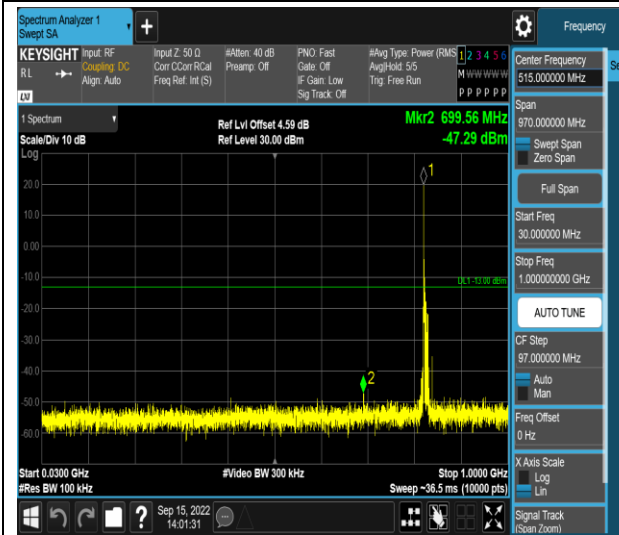
Band5-10MHz-QPSK-20525-1RB#0-Range1:30~1000MHz
