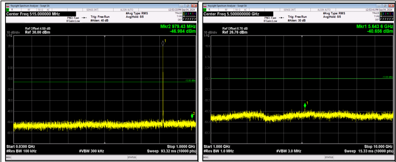
Band5-1.4MHz-QPSK-20525-1RB#0-Range1:30~1000MHz
