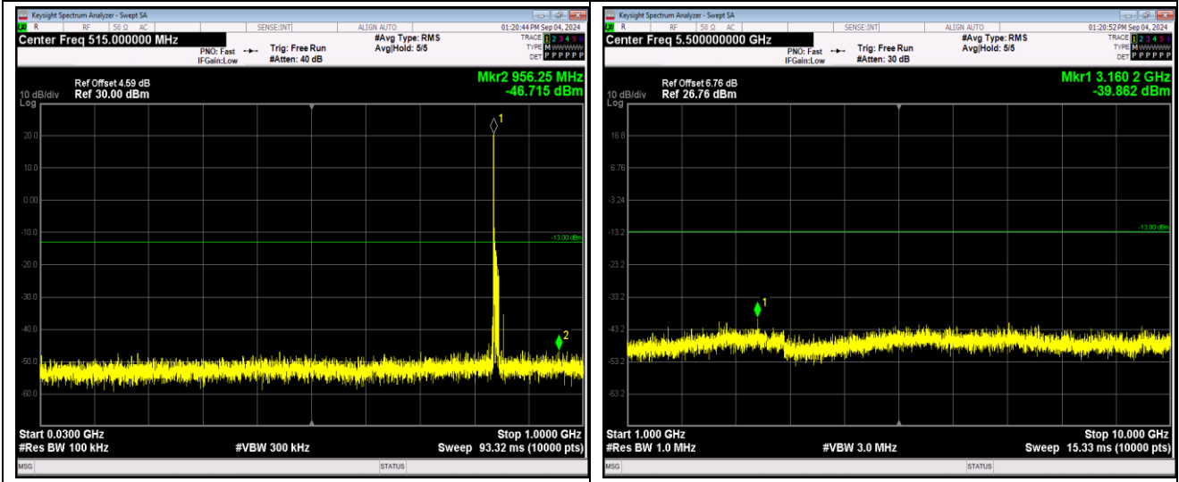
Band7-5MHz-QPSK-20775-1RB#0-Range1:30~1000MHz
