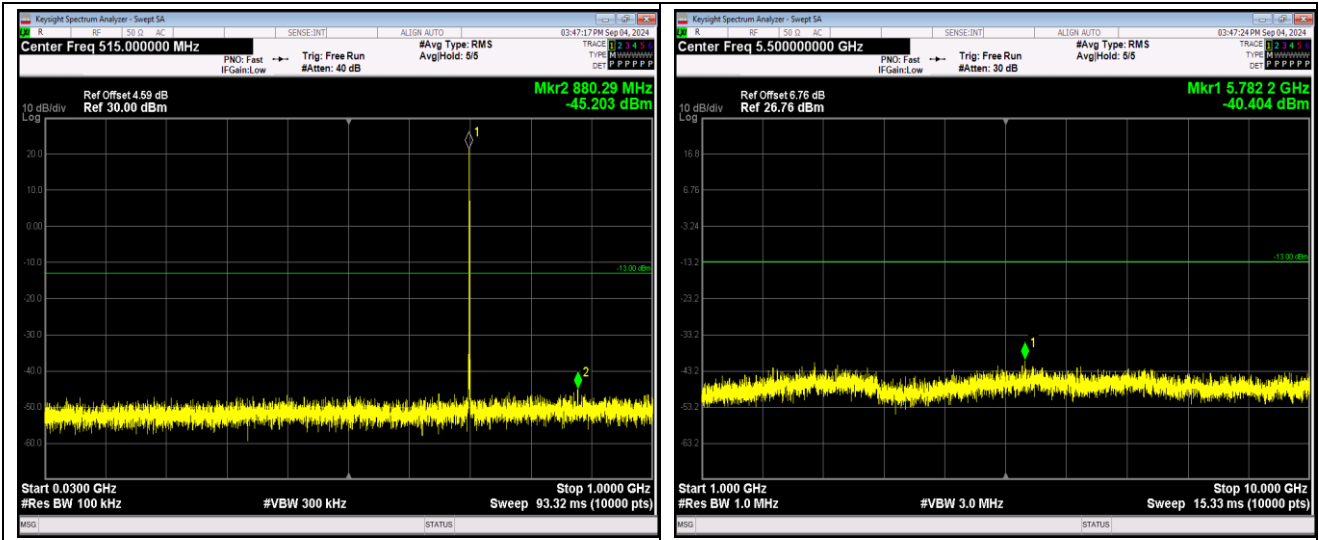
Band12-1.4MHz-QPSK-23173-1RB#0-Range1:30~1000MHz
