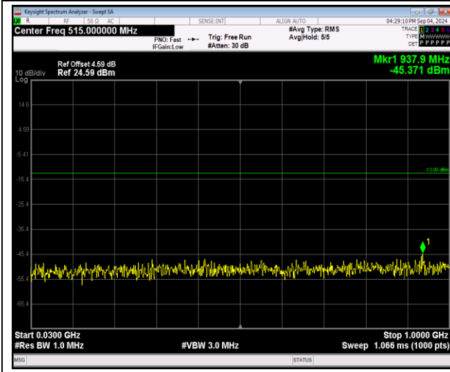
Band66-1.4MHz-QPSK-132322-1RB#0-Range1:30~1000MHz
