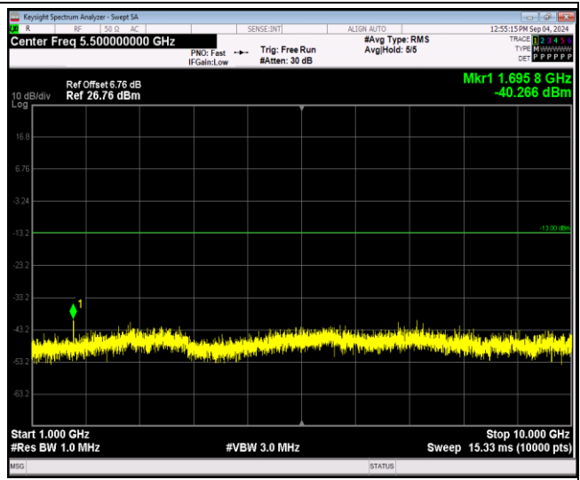
Band5-10MHz-QPSK-20450-1RB#0-Range2:1000~10000MHz
