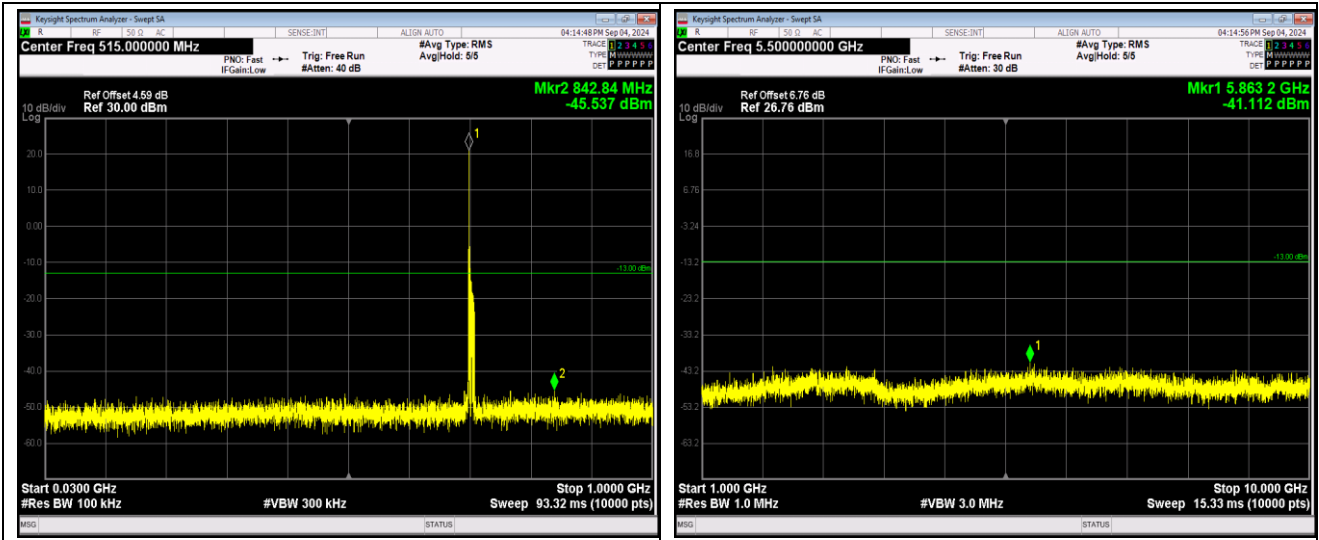
Band66-1.4MHz-QPSK-131979-1RB#0-Range1:30~1000MHz
