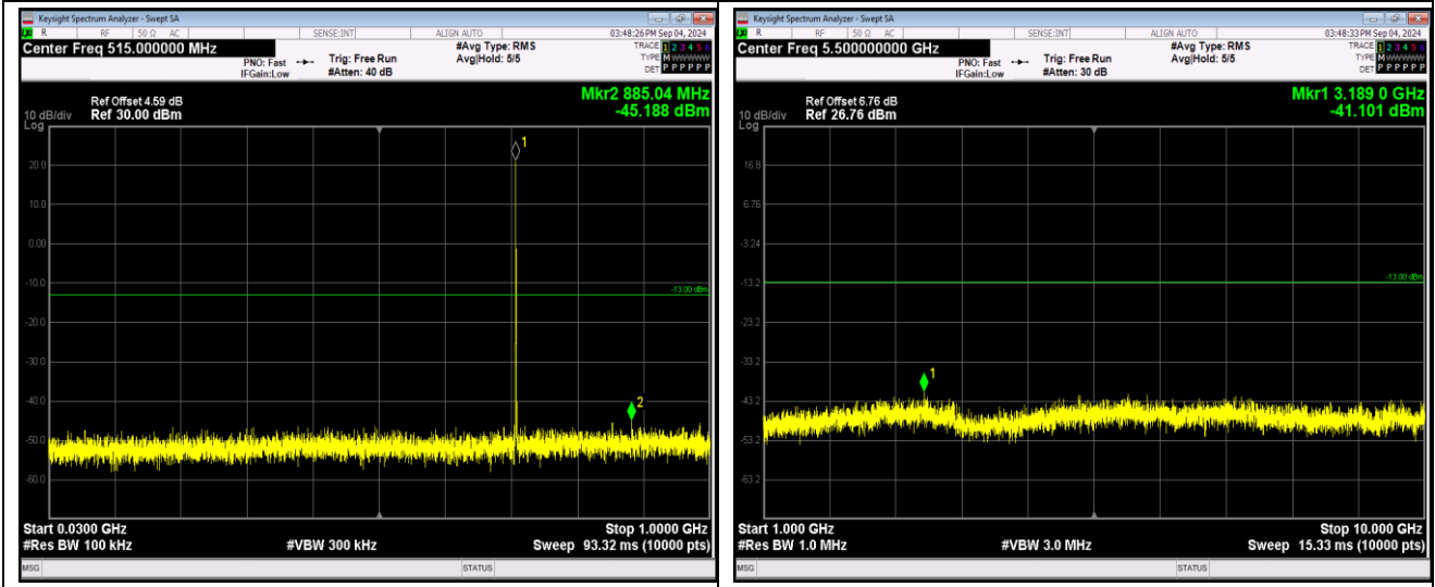
Band12-1.4MHz-16QAM-23017-1RB#0-Range1:30~1000MHz
