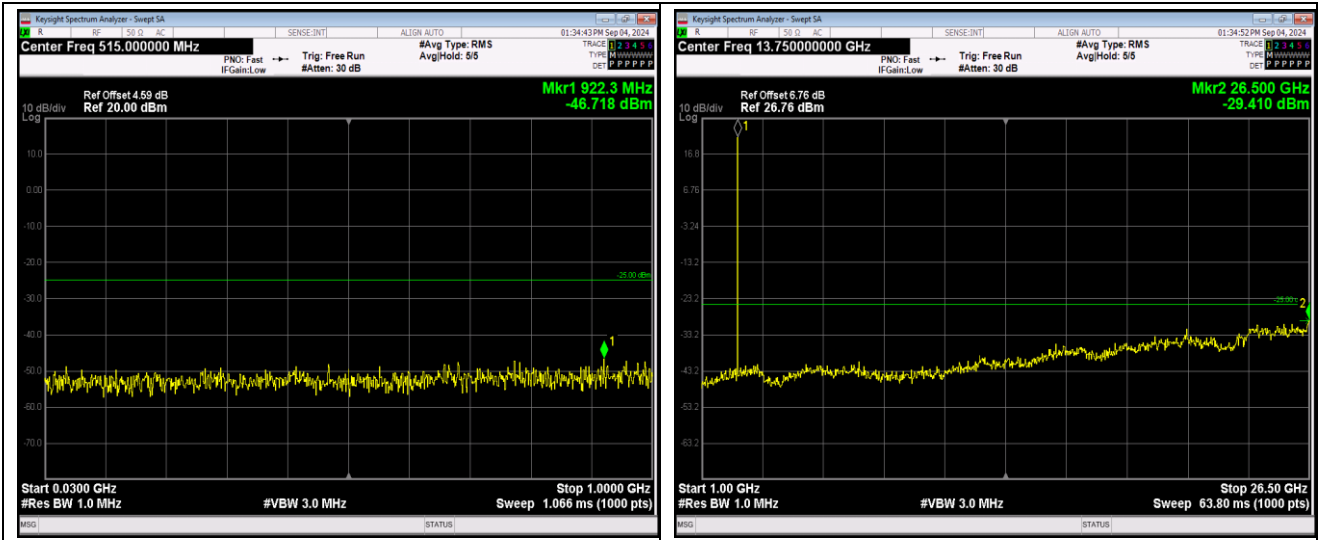
Band7-5MHz-16QAM-21100-1RB#0-Range1:30~100 0MHz
