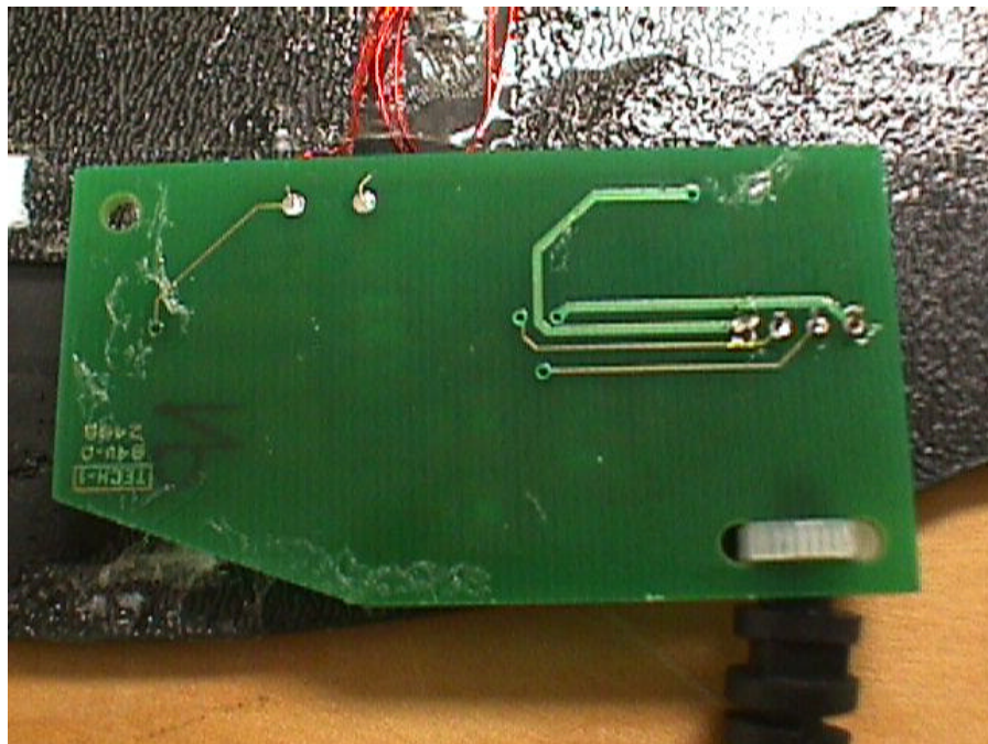
Mousepad, Processor Board, Solder Side
