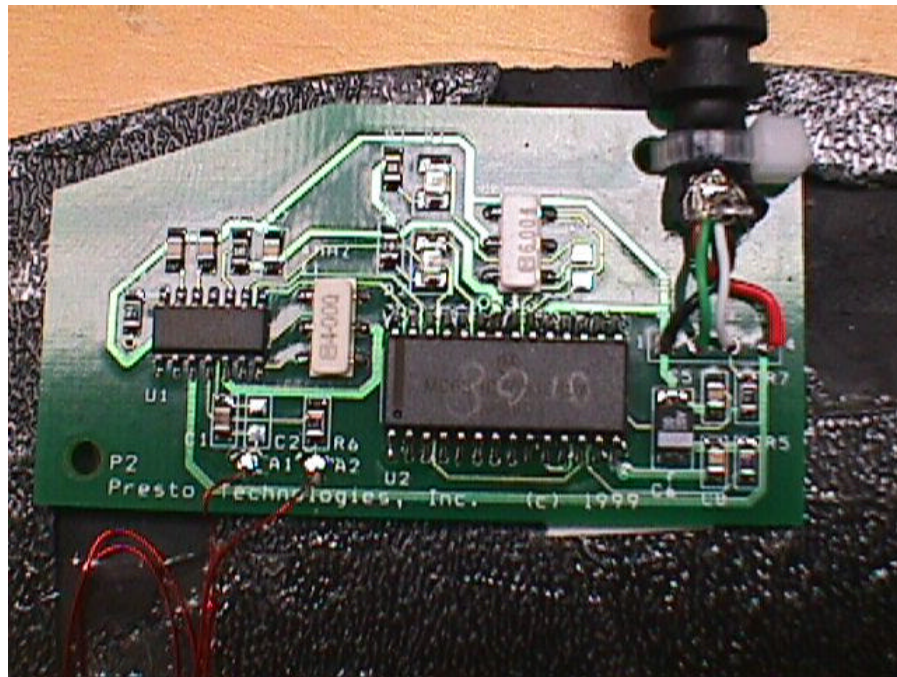
Mousepad, Processor Board, Component Side
