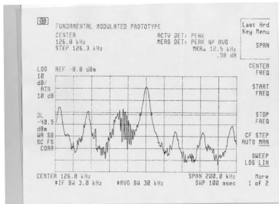
FIGURE 26: Mousepad wirewound antenna occupied bandwidth Plot 4
