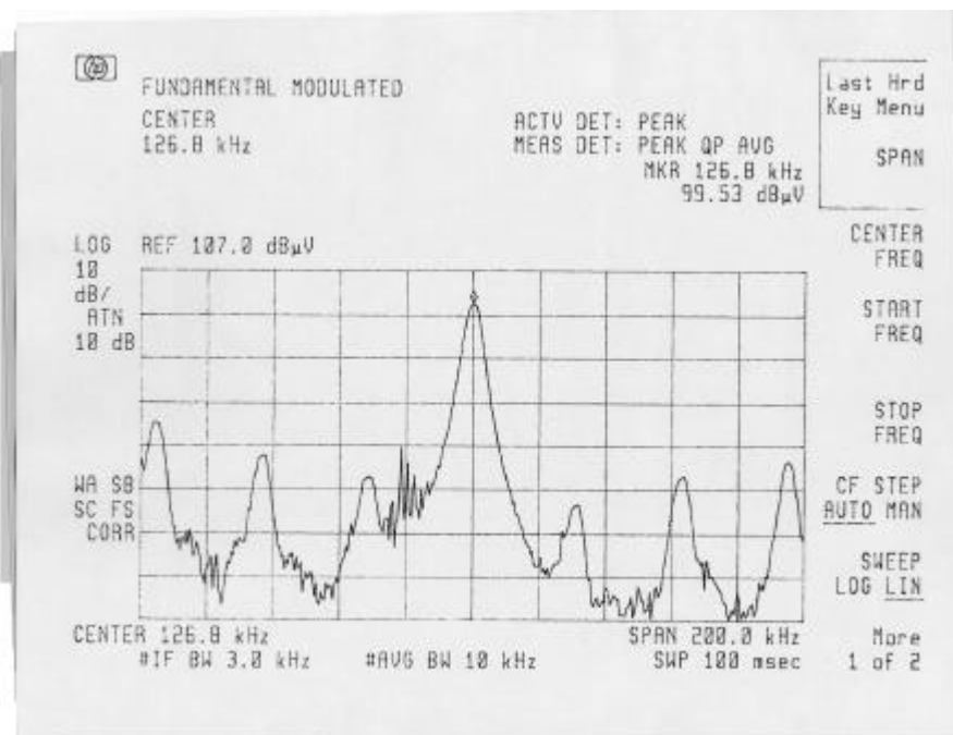
FIGURE 24: Mousepad etched PCB antenna occupied bandwidth Plot 2
