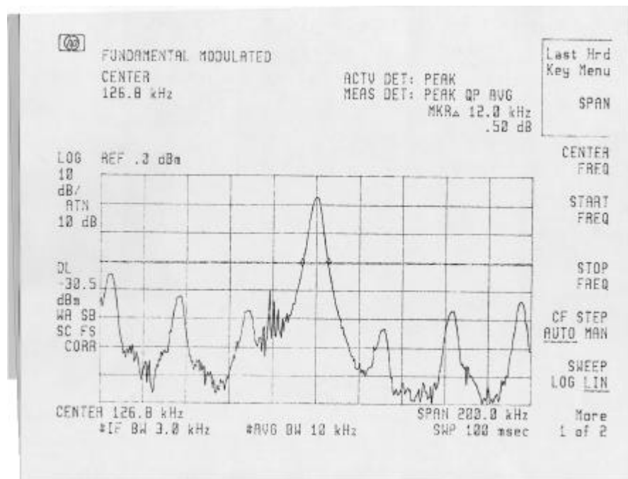
FIGURE 23: Mousepad Etched PCB antenna occupied bandwidth Plot 1
