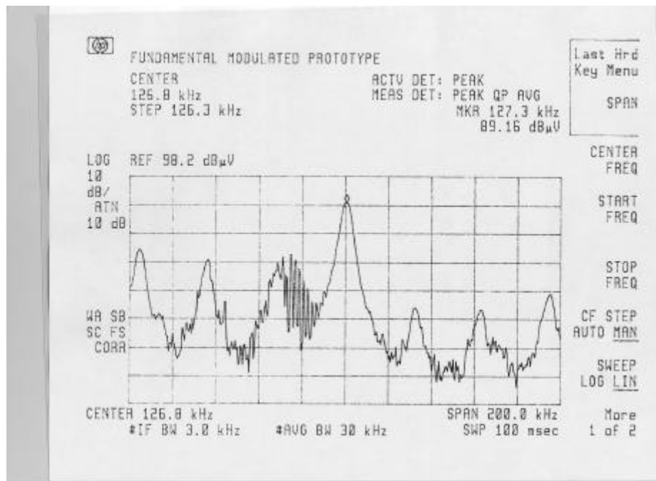
FIGURE 25: Mousepad wirewound antenna occupied bandwidth Plot 3
