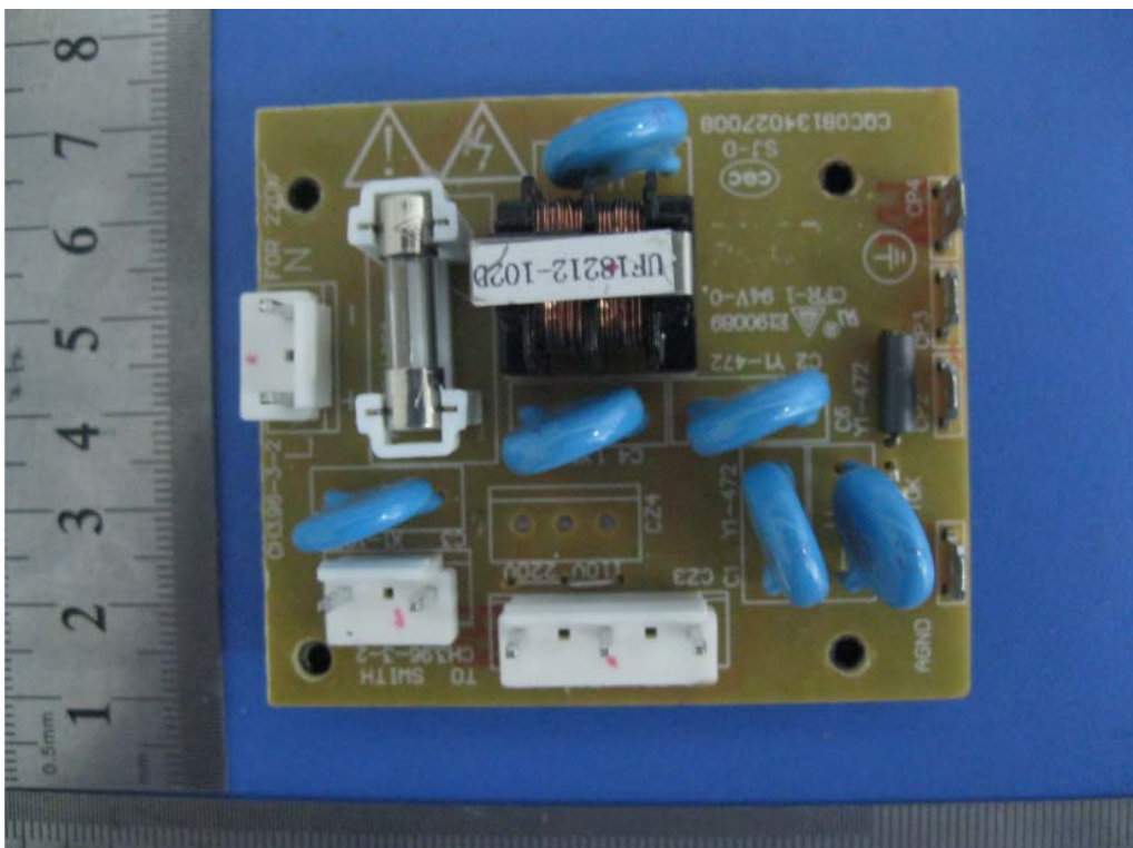
EUT- PCB Board 4 Front View
