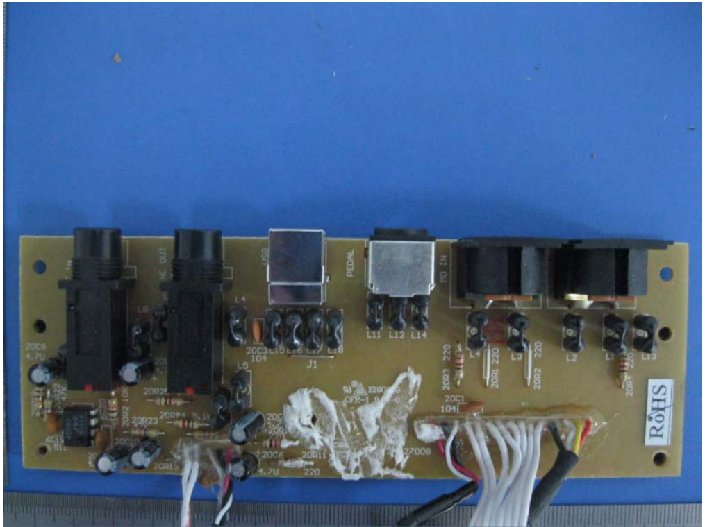
EUT- PCB Board 2 Front View
