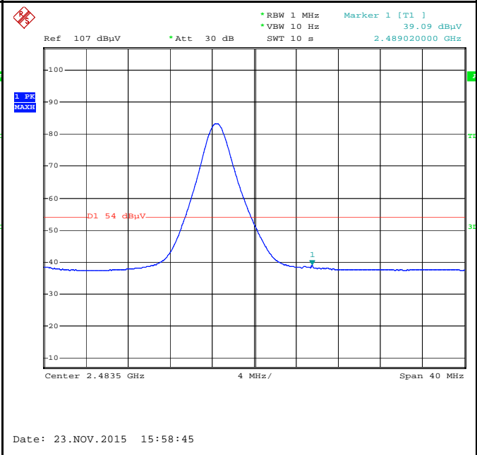
Band Edge, Right Side-AV
