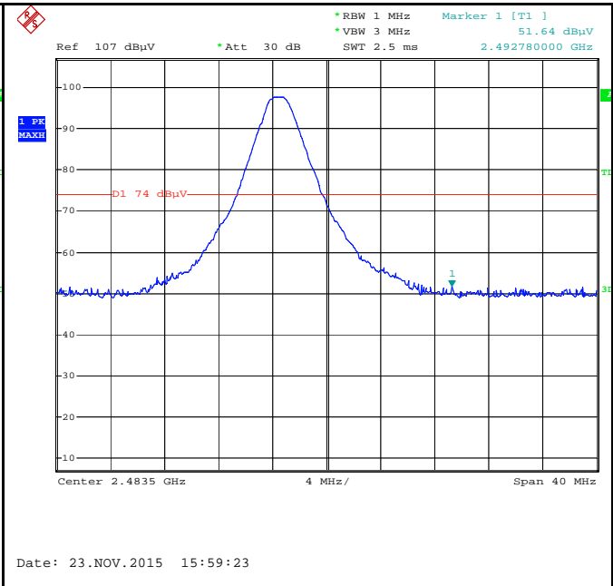
Band Edge, Right Side (Peak)
