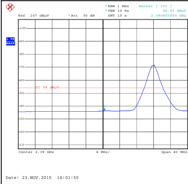
Band Edge, Left Side-AV
