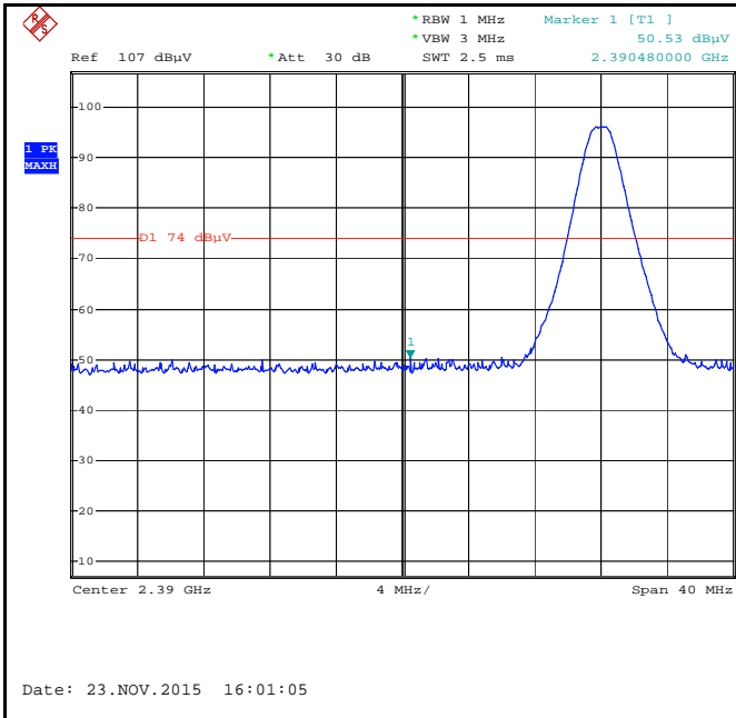
Band Edge, Left Side (Peak)
