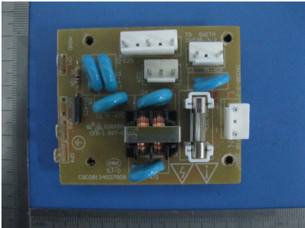
EUT- PCB Board 3 Front View
