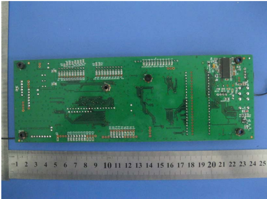
EUT- PCB Board 1 Rear View
