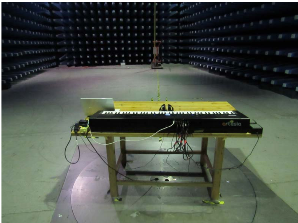
Radiated Emissions Setup Below 1GHz Rear View
