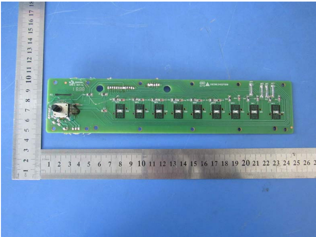
EUT PCBA 6 – Front View
