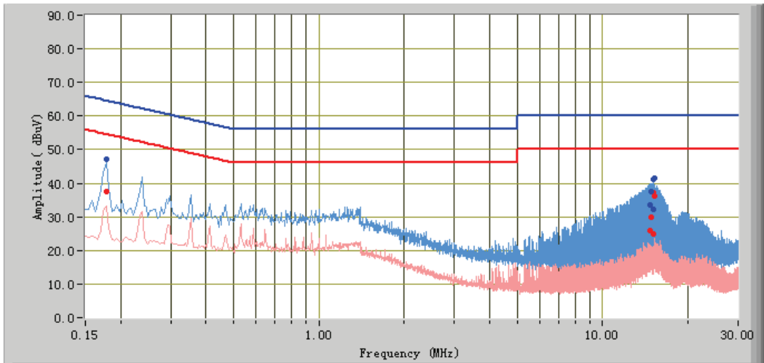
Phase Line Plot at 120Vac, 60Hz
