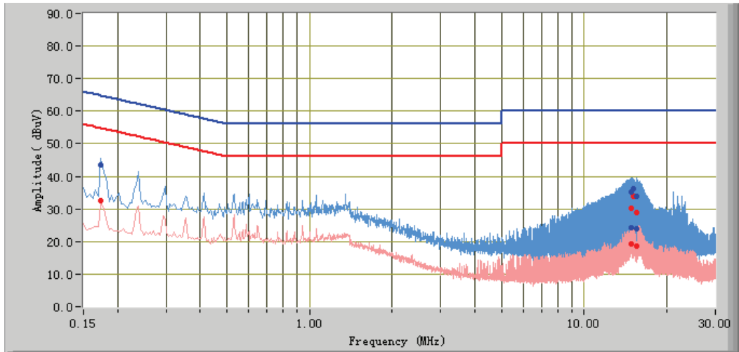
Phase Neutral Plot at 120Vac, 60Hz
