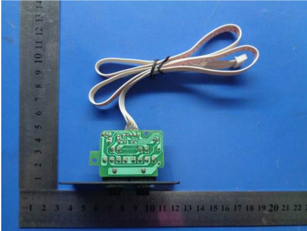
EUT PCB Board 7 - Rear View
