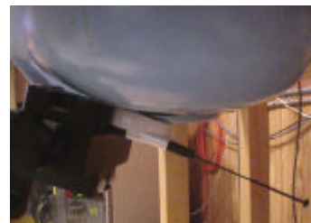
Figure 6. Head SAR Test Setup
