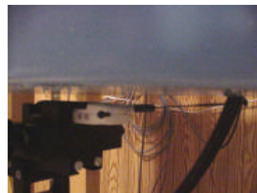
Figure 9. Body SAR Test Setup
