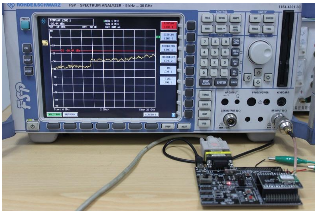
Photograph 3: Set-up for Conduct Power
