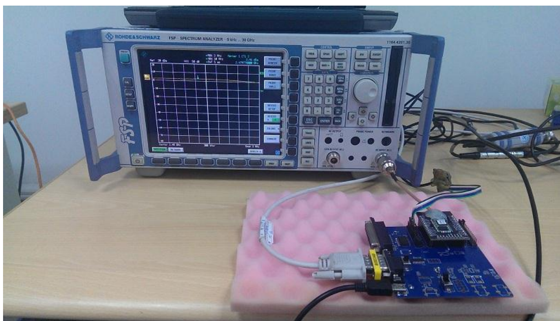
Photograph 3: Set-up for Conduct Power
