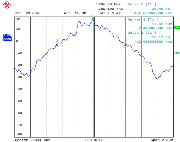
Figure 5: 20dB Bandwidth, Mode B (2441MHz)
