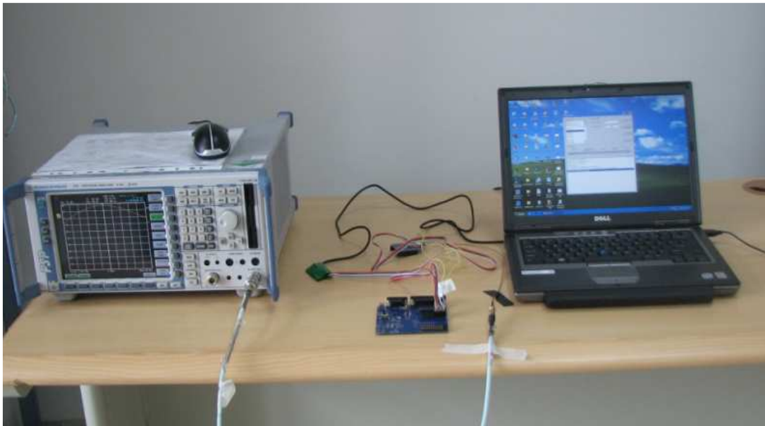
Photograph 1: Set-up for Conducted Emission at Antenna Port
