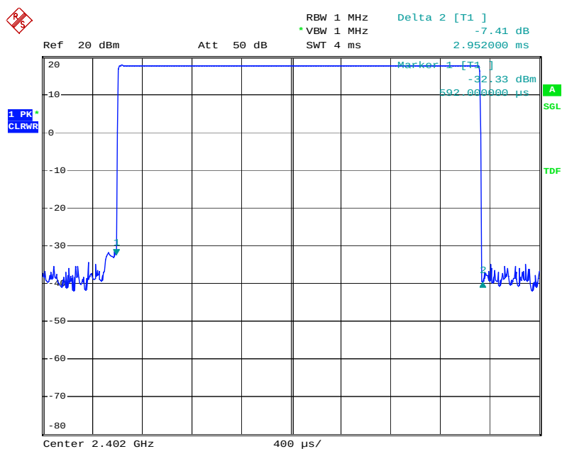
Figure 10: Dwell Time, Mode G (Hopping), DH5, Low channel
