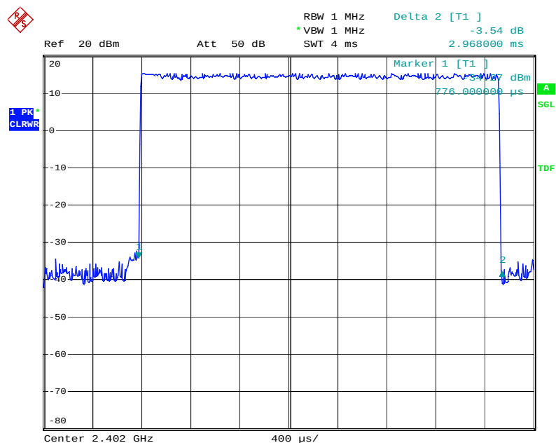
Figure 12: Dwell Time, Mode G (Hopping), 3-DH5, Low channel
