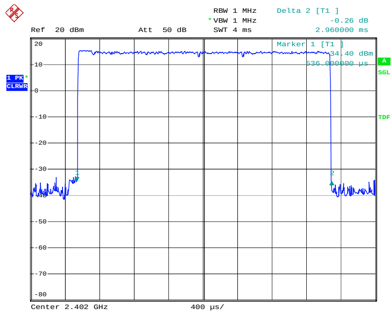
Figure 11: Dwell Time, Mode G (Hopping), 2-DH5, Low channel
