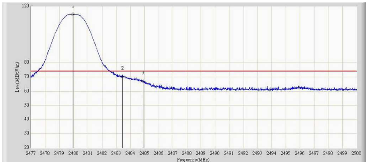
Figure 30: Band Edge Radiated Emission, Spectral Diagram, Mode C (2480MHz)
