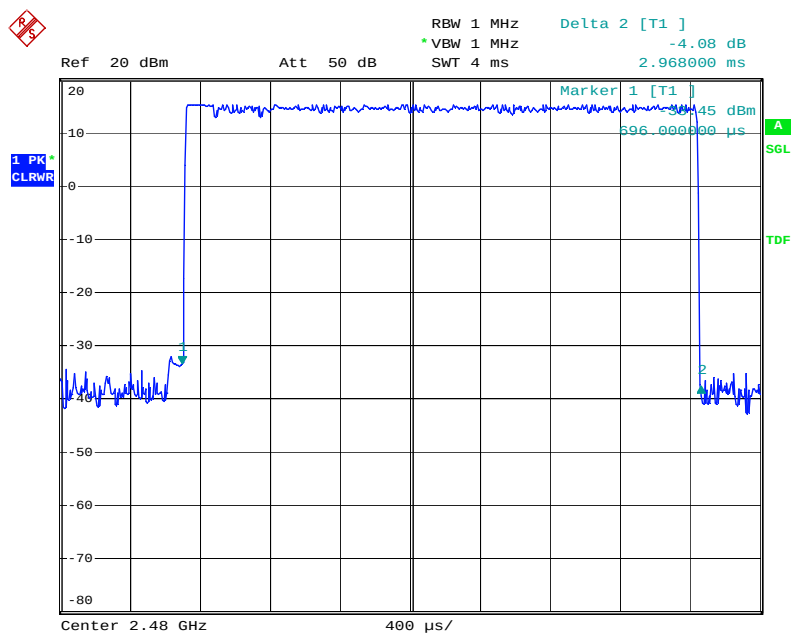
Figure 18: Dwell Time, Mode G (Hopping), 3- DH5, High channel
