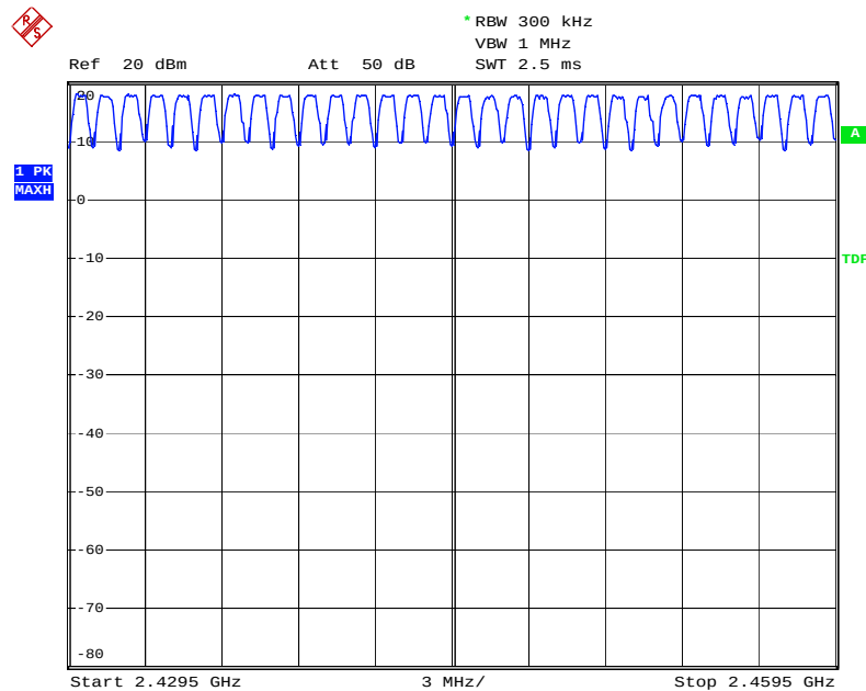
Figure 8: Hopping Frequencies up to 2459.5MHz, Mode G (Hopping)
