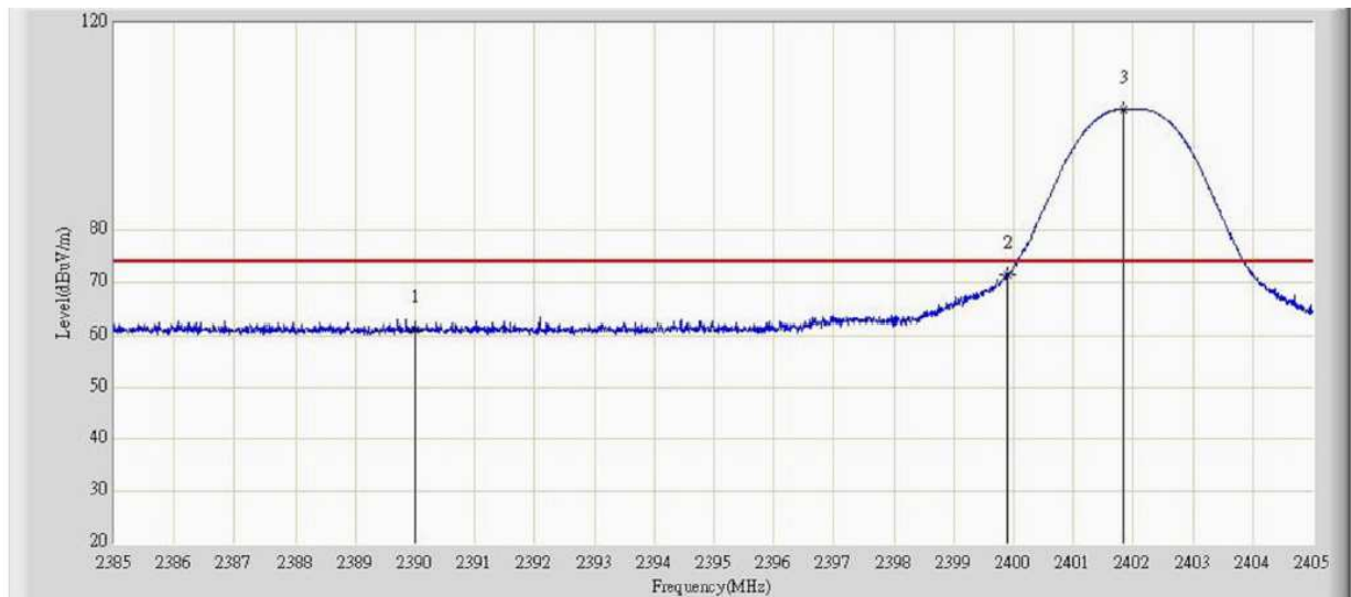
Figure 29: Band Edge Radiated Emission, Spectral Diagram, Mode A (2402MHz)
