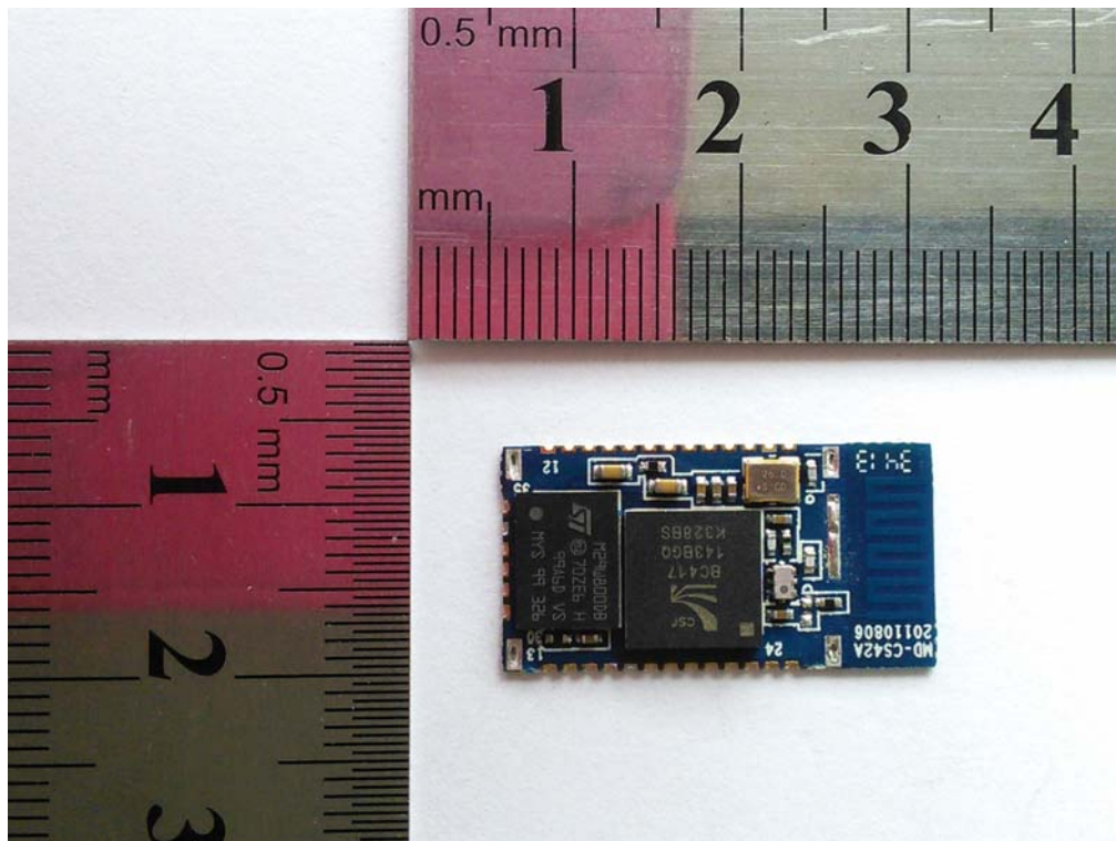
EUT – Front (without shielding) View
